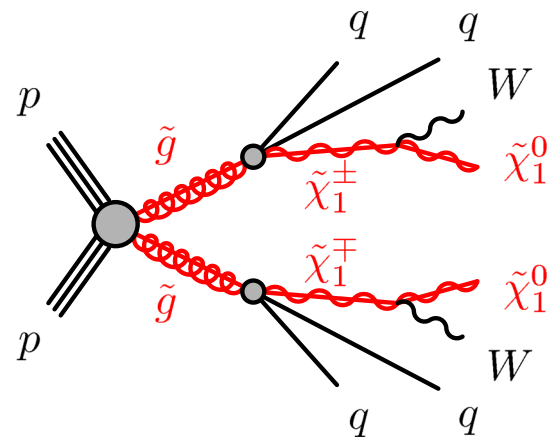
Fig. 1 The decay topology of the signal model considered in this search
