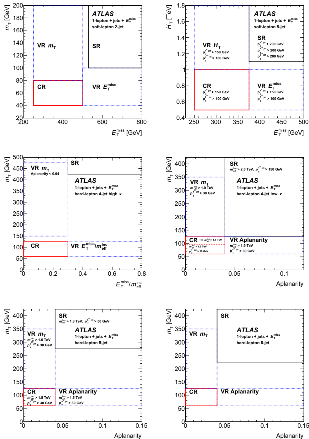
Fig. 2 Graphical illustration of the soft-lepton 2-jet ( top left ), soft-lepton 5-jet ( top right ), hard-lepton 4-jet high- x ( middle left ), 4-jet low- x ( middle right ), 5-jet ( bottom left ) and 6-jet ( bottom right ) signal (SR), control (CR) and validation (VR) regions. In addition to the two variables shown on the x and y axes, labels indicate other event selec-
