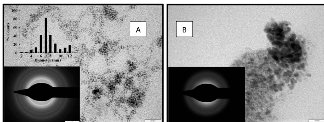
Figure 9. Effect of flow rate in continuous flow microreactor on the nanoparticle size and crystallinity as observed by TEM and Selected Area Electron Diffraction (SAED). (A) Flow rate= 14 µL/s and (B) flow rate = 28 µL/s (image scale: both TEM 20 nm, both SAED 5 nm) (reprinted with permission with Elsevier [85], 2016).
