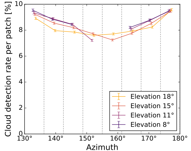
Figure 7. Cloud detection rate for each patch of the sky shown in Fig. 6.
