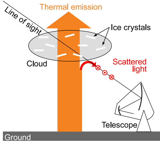
Figure 1. Illustration of the microwave signal from clouds. Ice crystals scatter thermal emission from the ground and generate horizontal polarization.
