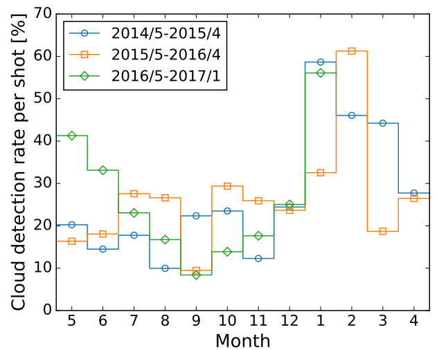
Figure 8. Annual variation of the cloud detection rate. Each line shows the result in the different year. The cloud detection rate increases in January and February every year because of Altiplanic winter.
