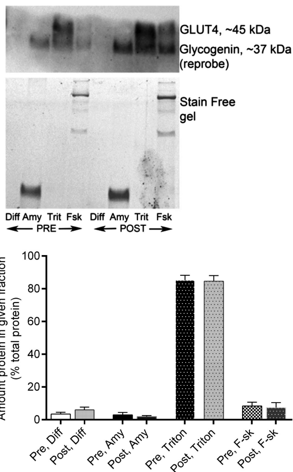
Figure 2. Representative blot of GLUT4 and glycogenin (top panel) and pooled data for GLUT protein content (expressed as % of total GLUT4 pool; bottom panel) in wash solutions (Diff, Amy and Triton) and skinned fibers (F-sk) before (PRE) and after (POST) exercise.
