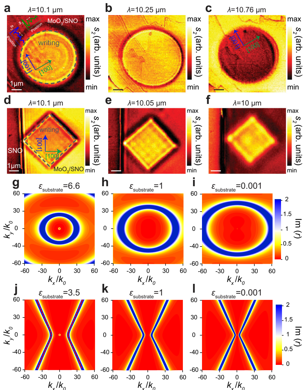
Fig. 5 | Tunable polaritonics with \alpha\text{-MoO}_3/\text{SNO} architectures. IR s-SNOM second harmonic near field experimental amplitude s_2 images of pristine \alpha\text{-MoO}_3/\text{SNO} at a \lambda = 10.1 \mu\text{m} , b \lambda = 10.25 \mu\text{m} , and c \lambda = 10.76 \mu\text{m} . The lithography pattern (a circle with 5 \mu\text{m} diameter) was made by applying 10 V potential at the c-AFM tip and a flake of 120 nm \alpha\text{-MoO}_3 is transferred on the top at parts ( a–c ). IR s-SNOM second harmonic near-field amplitude s_2 images of pristine \alpha\text{-MoO}_3/\text{SNO} at d \lambda = 10.1 \mu\text{m} , e \lambda = 10.05 \mu\text{m} , f \lambda = 10 \mu\text{m} , the lithography pattern (a square with 4 \mu\text{m} side) was made by applying 10 V potential at the c-AFM tip and a flake of 120 nm \alpha\text{-MoO}_3 is
