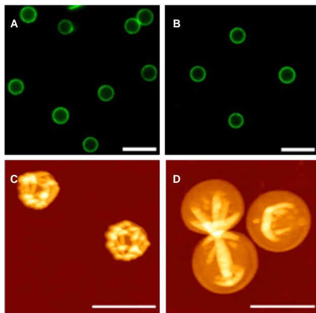
Figure 2. Fluorescence microscopy (top) and atomic force microscopy (bottom) images of L-PEToxTE (A, C) and B-PEToxAlk (B, D) capsules assembled on a sacrificial core of 2.78 \mu\text{m} diameter \text{SiO}_2 particles at pH 4 (NaOAc, 20 mM). Scale bars = 5 \mu\text{m} .
