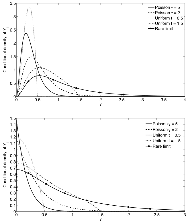
Fig. 4 Conditional density of Y_j , given that phase j = 4 is observed, for the two observation schemes with different parameter values, and the rare observation limit, as \alpha = [1, 0, 0, 0, 0] (top) and \alpha = [1/5, 1/5, 1/5, 1/5, 1/5] (bottom). The point mass at zero is clear when \alpha = [1/5, 1/5, 1/5, 1/5, 1/5] .
