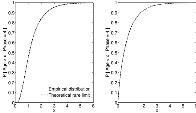
Fig. 7 . Comparison of the rare observation limit of the age distribution with the empirical limit computed by simulations, for \alpha = [1, 0, 0, 0, 0] (right) and \alpha = [1/5, 1/5, 1/5, 1/5, 1/5] (left), when the observed phase is j = 4 .
