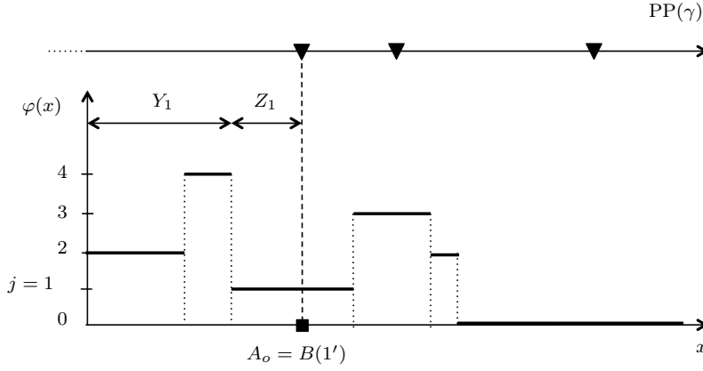
Fig. 1 A Possible trajectory of the phase process until absorption. The observation process is a Poisson process with rate \gamma (denoted as PP(\gamma) ), where the \blacktriangledown symbols represent the events, and the phase is j = 1 at the first observation event.
