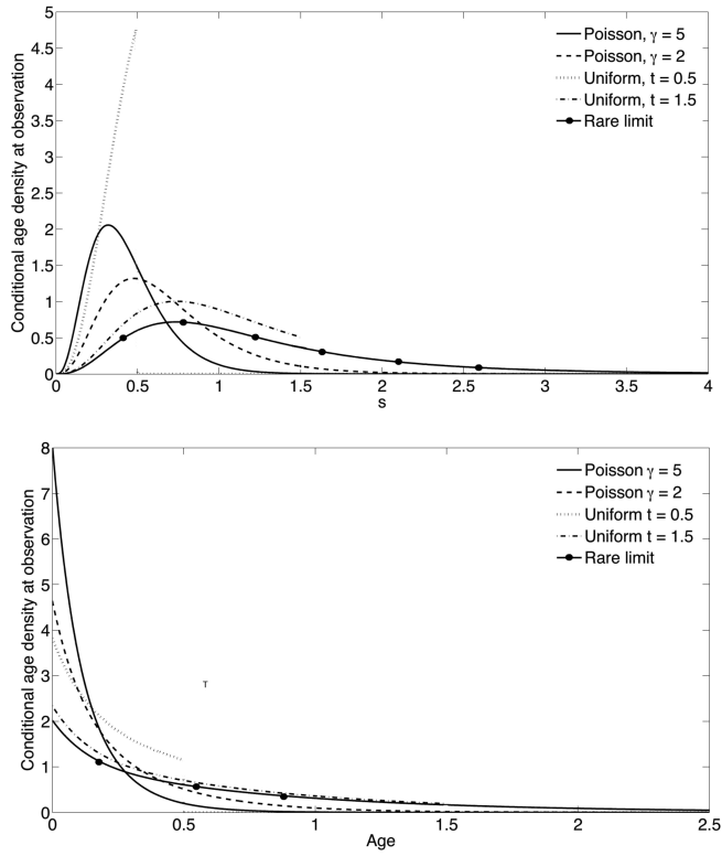
Fig. 3 Conditional age density at the observation time, given that phase j = 4 is observed, for the two observation schemes with different parameter values, and the rare observation limit, as \alpha = [1, 0, 0, 0, 0] (top) and \alpha = [1/5, 1/5, 1/5, 1/5, 1/5] (bottom).
