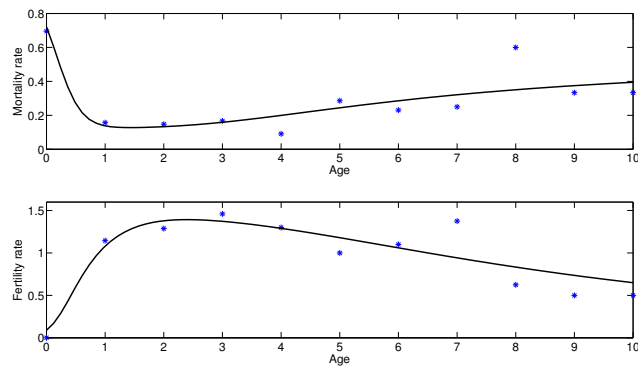
Fig. 8 Estimated age-specific mortality and fertility rates (stars), and the age-specific mortality and fertility curves computed with the optimal Markovian model fitting the data (plain lines).
