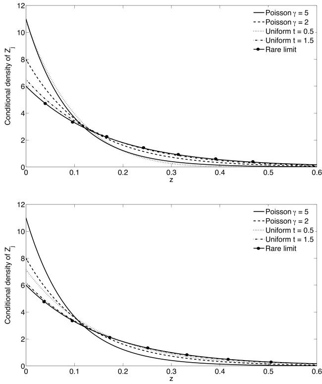
Fig. 5 Conditional density of Z_j , given that phase j = 4 is observed, for the two observation schemes with different parameter values, and the rare observation limit, as \alpha = [1, 0, 0, 0, 0] (top) and \alpha = [1/5, 1/5, 1/5, 1/5, 1/5] (bottom).
