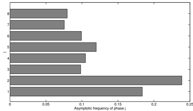
Fig. 9 The asymptotic phase frequency in the MBT modelling the Chatham Island black robin population, if the population evolves with the demographic rates of 2007-2014.
