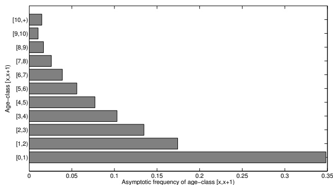
Fig. 10 The asymptotic age frequency in the Chatham Island black robin population if the population evolves with the demographic rates of 2007-2014.
