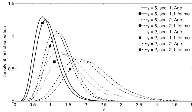
Fig. 6 Conditional age/lifetime density at the time of the last Poisson observation when the observed sequence is 1, 2, 3, 3, 4 (Sequence 1) and 2, 3, 1, 1, 4 (Sequence 2), with \alpha = [1, 0, 0, 0, 0] .
