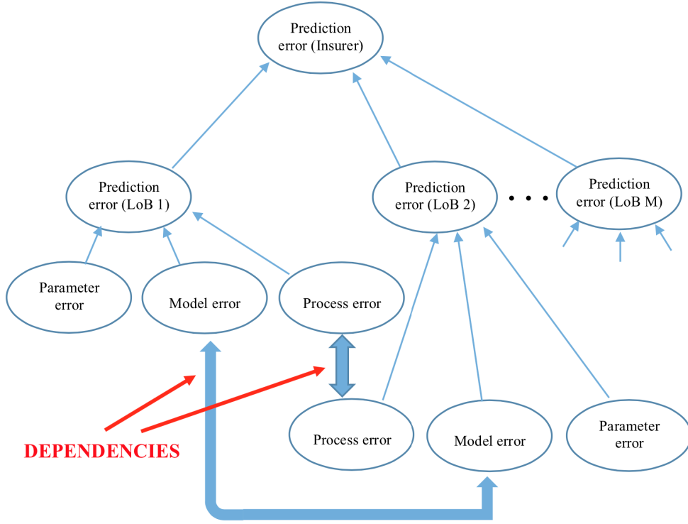
Figure 5.2: Structure of dependencies between components of prediction error
