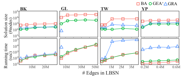
Figure 7: Scalability analysis by varying LBSN size
