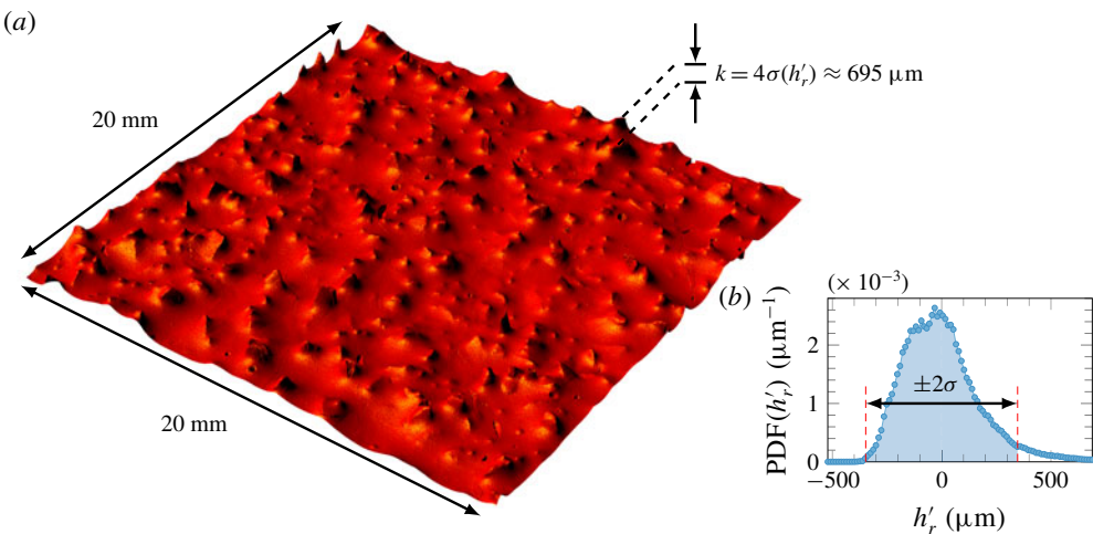
FIGURE 2. (a) Height scan captured using confocal microscopy of a patch of sandpaper of size 20 mm \times 20 mm with a resolution of 2.5 \mu\text{m} . The typical size of the grains is given by k \equiv 4\sigma(h_r) = 695 \mu\text{m} where h_r is the height and \sigma the standard deviation. The normalized typical grain size is then k/d \approx 0.01 . (b) Probability density function (PDF) of the measured height of the roughness stripe, with subtracted mean h'_r = h_r - \langle h_r \rangle .
