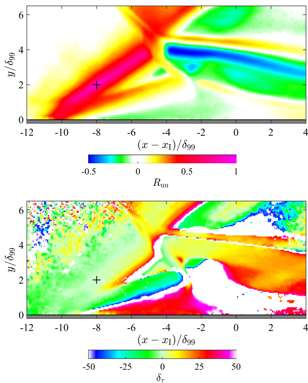
Fig. 16 Spatial distribution of the amplitude of the maximum correlation for the horizontal velocity component in the field of view compared to the reference point at (x - x_I)/\delta_{99} = -8.0 and y/\delta_{99} = 2.0 (top) and the corresponding time shift at which the correlation coefficient is strongest (bottom)
