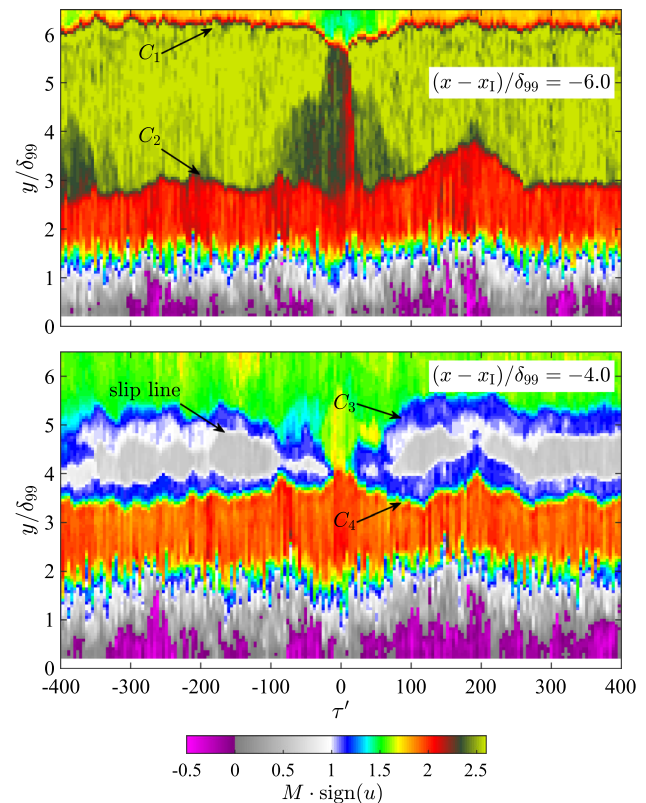
Fig. 7 Temporal development of the Mach number along vertical lines before the shock interaction at (x - x_1)/\delta_{99} = -6.0 (top) and downstream of it at (x - x_1)/\delta_{99} = -4.0 (bottom). At the time \tau' = 0 , the shock reflection type has changed from Mach reflection to a regular reflection
