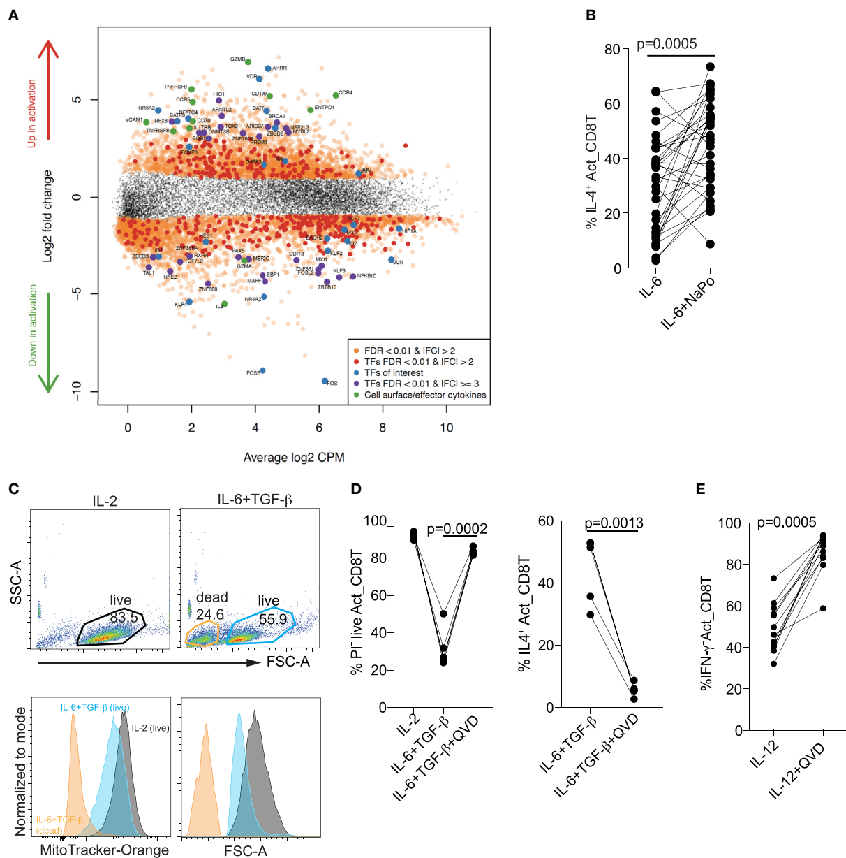
FIGURE 6 | Differentiation of “T C 2” cells is associated with increased fatty acid metabolism and is caspase dependent. (A) Mean-difference plot showing changes in gene expression associated with “T C 2” differentiation. (B) IL-4 expression is increased with supplementation of sodium propionate (NaPo) (right). (C) Decreased mitochondrial membrane potential (MitoTracker-Orange stain) and cellular size in live “T C 2” compared with T C 1 cells. Data are representative of n > 10 donors, all with similar results. (D) Prevention of cell death and IL-4 expression at day 5 by the caspase inhibitor QVD-Oph added at day 0 and supplemented at day 3. (E) Enhancement of IFN- \gamma expression at day 5 by the caspase inhibitor QVD-Oph added at day 0 and supplemented at day 3. P -values were calculated by Wilcoxon matched-pairs signed rank test.
