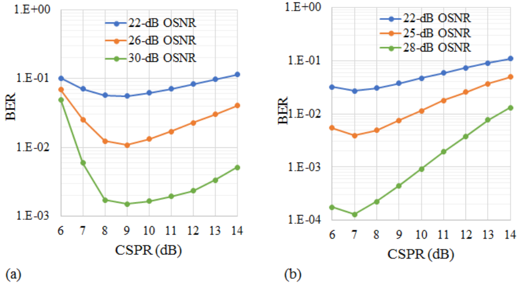
Fig. 4.8 BER versus CSRR for 25-Gbaud signals (a) with 5% frequency gap, (b) with 20% frequency gap.
