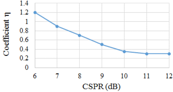
Fig. 4.14 Scaled coefficient \eta used in the experimental demonstration versus CSRR.
