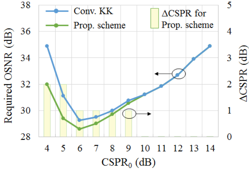
Fig. 5.7 Required OSNR and optimal \Delta CSCR as a function of original CSCR in the bth configuration.
