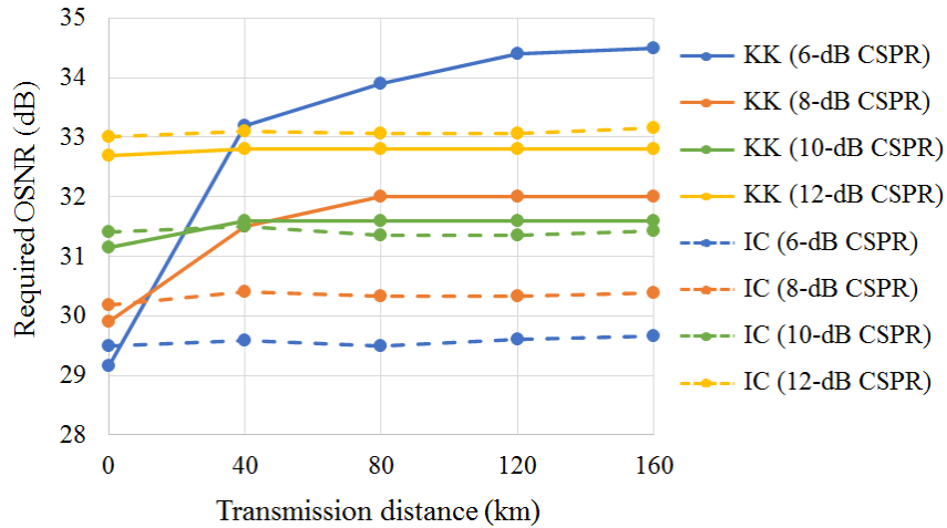
Fig. 3.14 Required OSNR versus transmission distance for both KK and IC receiver (@BER= 1.0 \times 10^{-3} ).
