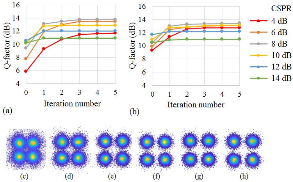
Fig. 3.11 Q-factor as a function of iteration number at btb for (a) OFDM, and (b) single-carrier signals with various CSRs. (c-h) are the OFDM signal constellations without the iterative cancellation and with 1-, 2-, 3-, 4-, 5-times iterations, respectively.
