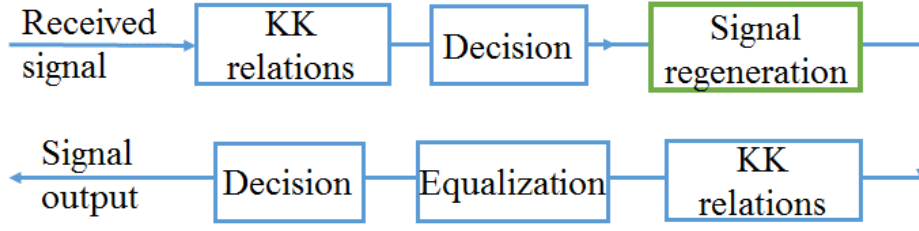
Fig. 5.6 DSP flow chart for the proposed virtual CSCR enhancement scheme.
