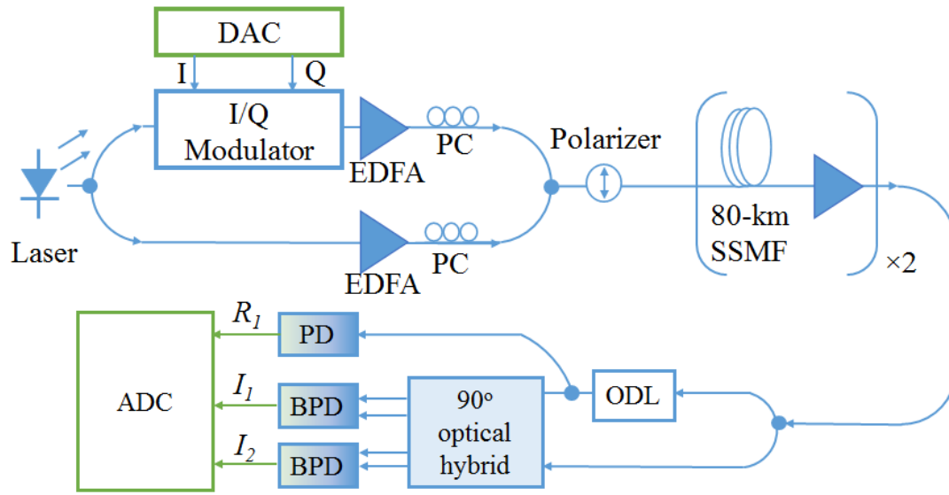
Fig. 4.13 Experimental setup for CADD scheme.
