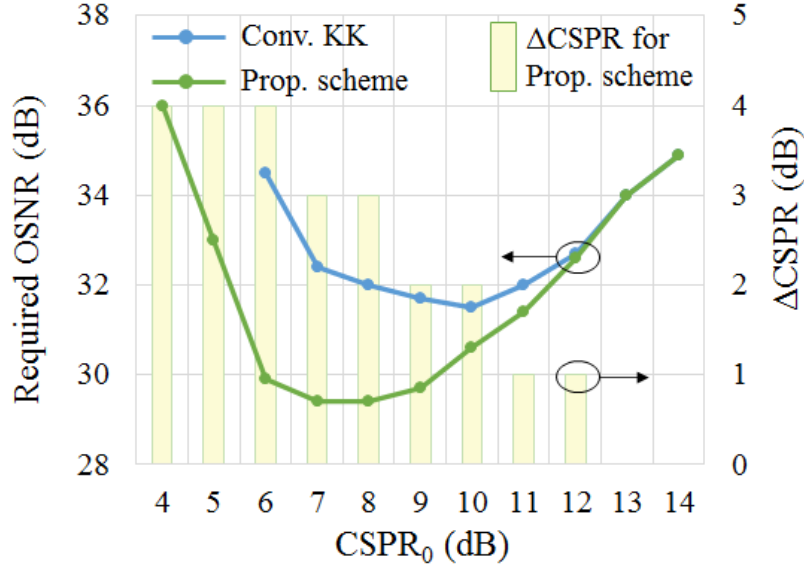
Fig. 5.8 Required OSNR and optimal \Delta CSPR as a function of original CSPR after 160-km transmission.
