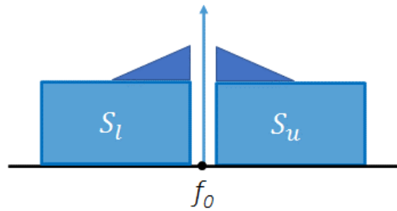
Fig. 5.11 Schematic diagram of triangular power loading scheme. S_l and S_u are lower and upper sideband signals, respectively.
