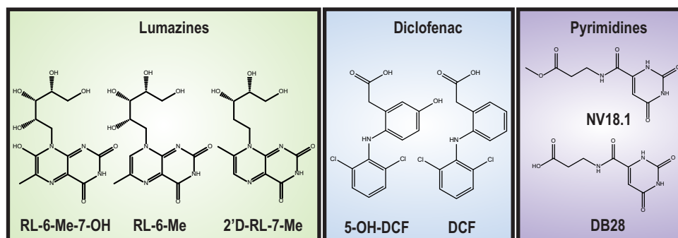
Figure 3. Chemical structures of MR1-restricted ligands. Pterin-based ligands: 6-formylpterin (6-FP) and acetyl-6-formylpterin (Ac-6-FP) (9); pyrimidine-based ligands: 5-(2-oxopropylideneamino)-6-D-ribitylaminouracil (5-OP-RU), 2’D-5-OP-RU, 3’D-5-OP-RU, ribityl-less analog 3-[(2,6-dioxo-1,2,3,6-tetrahydropyrimidin-4-yl)formamido]propanoic acid (DB28), and NV18.1 (17, 18); lumazine-based ligands: 7-hydroxy-6-methyl-8-D-ribityllumazine (RL-6-Me-7-OH), 6-methyl-8-D-ribityllumazine (RL-6-Me), and 2’D-RL-7-Me (9, 32); benzaldehyde-based ligand: 2-hydroxy-5-methoxybenzaldehyde (HMB) (16); salicylate-based ligand: salicylate 3-formylsalicylic acid (3-F-SA) (16); and the diclofenac-derived ligands: diclofenac (DCF) and 5-OH-DCF (16). MR1, MHC-I related protein 1.
