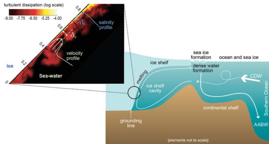
Figure 5. Schematic of microscale circulation processes on the Antarctic continental shelf. Grounded ice sheets are buttressed by floating ice shelves. Their basal melting is driven by the supply of salinity and heat from the Southern Ocean via CDW and its derivatives and influences the formation of deep-water masses and Antarctic Bottom Water (AABW). Zoomed view of boundary layer processes by showing snapshot of simulated turbulent dissipation (log scale) field underneath a sloping ice shelf base (Mondal et al., 2019).
