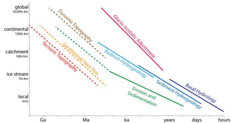
Figure 9. Earth processes and time scales. Illustrative plot showing typical length and time scale for ice sheet interactive processes at the base of the ice sheet. Template-setting (see text) interactions (dashed lines) occur over time scales of millions of years and direct interactions (solid lines) are short-term processes that result in a dynamic relationship between the ice sheet and surface processes of the solid Earth. Under typical conditions, these processes operate on length and time scales below and left of the line. Note the different scaling of the solid Earth processes relative to the surface processes. Threshold responses are not represented.
