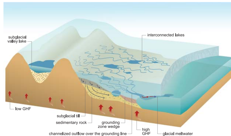
Figure 14. Basal hydrology and fluid-interchange processes. Schematic showing channelized subglacial drainage network (after Ashmore & Bingham, 2014) beneath a major ice stream. The cross section shows subglacial lakes and channels, and active subglacial hydrogeology in sedimentary sequences. A basal channel in the ice shelf cavity reflects a localized input of fresh meltwater to the cavity that will impact on the sub-ice-shelf melt rates, particularly at the grounding line, which will in turn affect the ice stream behavior (e.g., Le Brocq et al., 2013). Red arrows represent variable geothermal heat flux (GHF) interacting with the base of the ice sheet to produce meltwater.
