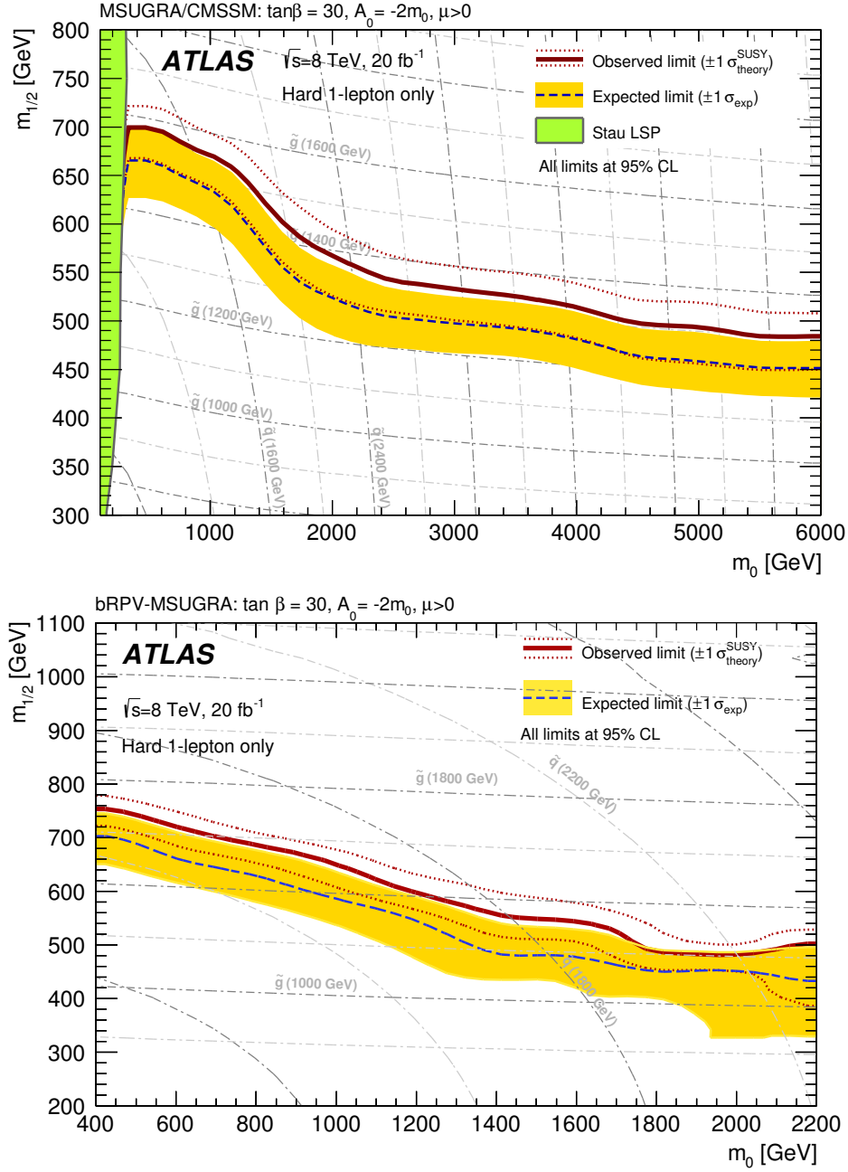
Figure 15. 95% CL exclusion limit from the hard single-lepton channel in the (m_0, m_{1/2}) plane for the mSUGRA/CMSSM model with \tan\beta=30 , A_0=-2m_0 and \mu>0 (top) and in the same plane for the bRPV model (bottom). The green area represents the region of the parameter space for which the stau is the LSP. The dark blue dashed line shows the expected limits at 95% CL, with the light (yellow) bands indicating the \pm 1\sigma variation on the median expected limit due to the experimental and background-only theory uncertainties. The observed nominal limit is shown by a solid dark red line, with the dark red dotted lines indicating the \pm 1\sigma variation on this limit due to the theoretical scale and PDF uncertainties on the signal cross section. Lines of constant squark and gluino masses are also shown.
