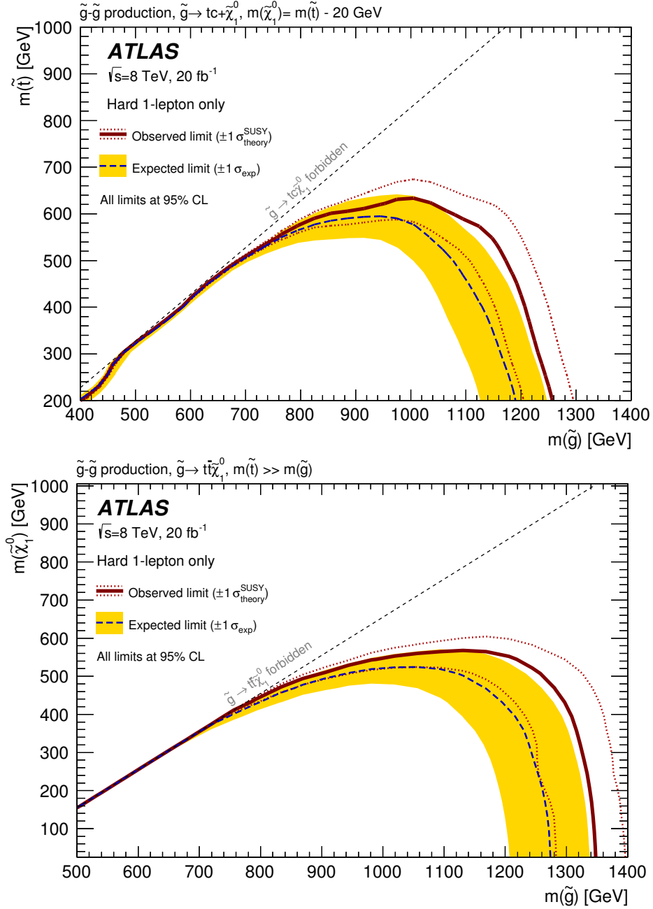
Figure 18. 95% CL exclusion limit from the hard single-lepton channel in the (m_{\tilde{g}}, m_{\tilde{\chi}_1^0}) plane for the simplified model with gluino-mediated top squark production, where the top squark is assumed to decay exclusively via \tilde{t} \rightarrow c\tilde{\chi}_1^0 (top) or where the gluinos are assumed to decay exclusively through a virtual top squark, \tilde{g} \rightarrow t\bar{t}\tilde{\chi}_1^0 (bottom). The dark blue dashed line shows the expected limits at 95% CL, with the light (yellow) bands indicating the \pm 1\sigma variation on the median expected limit due to the experimental and background-only theory uncertainties. The observed nominal limit is shown by a solid dark red line, with the dark red dotted lines indicating the \pm 1\sigma variation on this limit due to the theoretical scale and PDF uncertainties on the signal cross section.
