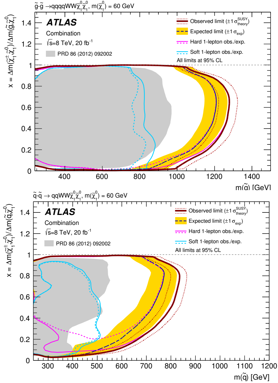
Figure 20. 95% CL exclusion limit for the gluino simplified model (top) and the first- and second-generation squark simplified model (bottom) from the combination of the soft and hard single-lepton analyses. The limits are presented in the (m_{\tilde{g}(\tilde{q})}, x) mass plane, where x = (m_{\tilde{\chi}_1^\pm} - m_{\tilde{\chi}_1^0}) / (m_{\tilde{g}(\tilde{q})} - m_{\tilde{\chi}_1^0}) , for the case in which the chargino mass is varied and the LSP mass is set at 60 GeV. The dark blue dashed line shows the expected limits at 95% CL, with the light (yellow) bands indicating the \pm 1\sigma variation on the median expected limit due to the experimental and background-only theory uncertainties. The observed nominal limit is shown by a solid dark red line, with the dark red dotted lines indicating the \pm 1\sigma variation on this limit due to the theoretical scale and PDF uncertainties on the signal cross section. The observed limit set by the previous ATLAS analysis [22] using 7 TeV data is shown as a gray area. The light blue and purple full (dashed) lines show the observed (expected) exclusion obtained by the soft and hard single-lepton analyses, respectively.
