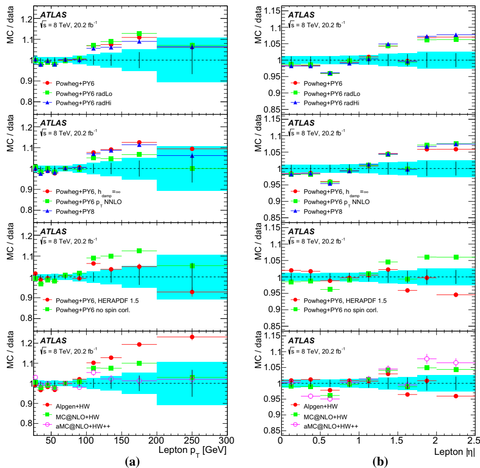
Fig. 9 Ratios of predictions of normalised differential cross-sections to data as a function of a p_T^\ell and b |\eta^\ell| . The data statistical uncertainties are shown by the black error bars around a ratio of unity, and the
