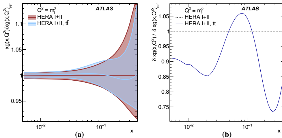
Fig. 15 a Ratio of the gluon PDF determined from the fit using HERA I+II data plus the normalised differential cross-section distributions as a function of |\eta^\ell| , |y^{e\mu}| and E^e + E^\mu in t\bar{t} events, to the gluon PDF determined from the fit using HERA I+II data alone, as a function of Bjorken- x . The uncertainty bands are shown on the two PDFs as the
