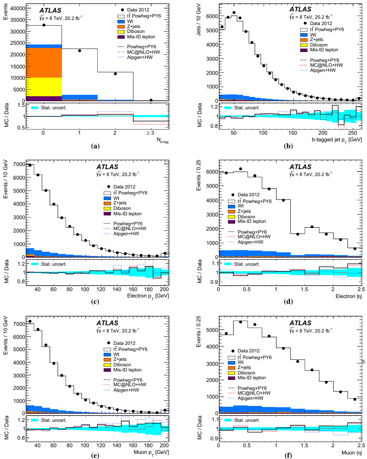
Fig. 1 Distributions of a the number of b -tagged jets in preselected opposite-sign e\mu events; and b the p_T of b -tagged jets, c the p_T of the electron, d the |\eta| of the electron, e the p_T of the muon and f the |\eta| of the muon, in events with an opposite-sign e\mu pair and at least one b -tagged jet. The reconstruction-level data are compared to the expectation from simulation, broken down into contributions from t\bar{t} (POWHEG + PYTHIA6), single top, Z +jets, dibosons, and events with
