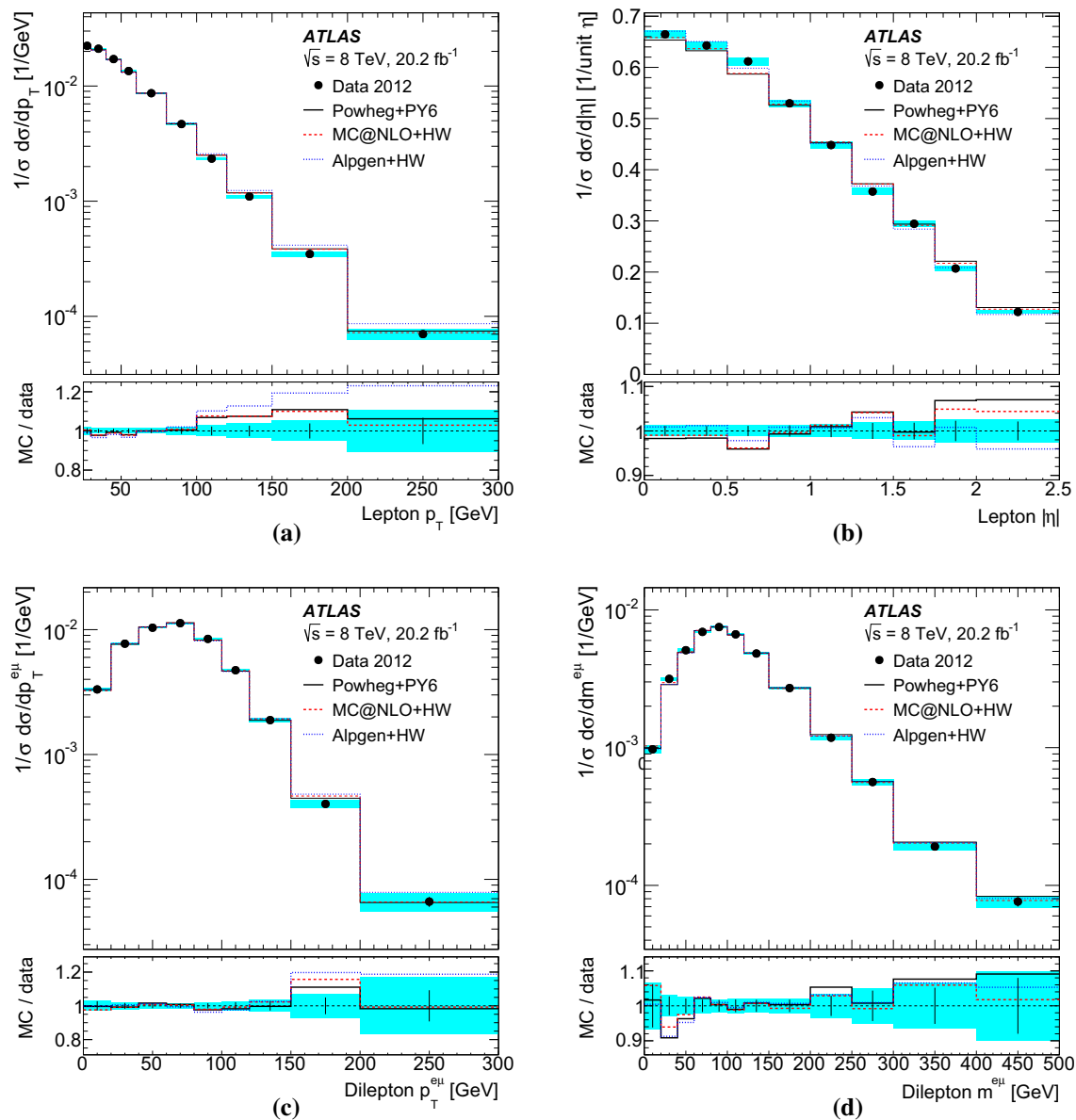
Fig. 7 Normalised differential cross-sections as a function of a p_T^\ell , b |\eta| , c p_T^{e\mu} and d m^{e\mu} . The measured values are shown by the black points with error bars corresponding to the data statistical uncertainties and cyan bands corresponding to the total uncertainties in each bin, and include the contributions via W \rightarrow \tau \rightarrow e/\mu decays. The
