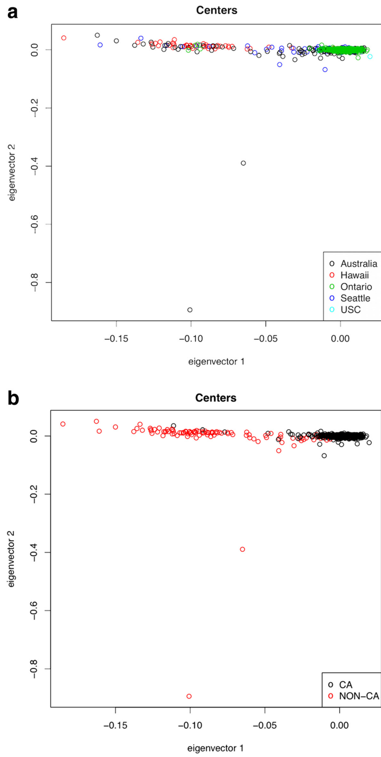
Fig. 3 a and b. PCA analysis of the population based samples. a. PCAs colored by CCFR center. b. PCAs colored by race with all non-Caucasian individuals colored in red and Caucasian samples colored in black
