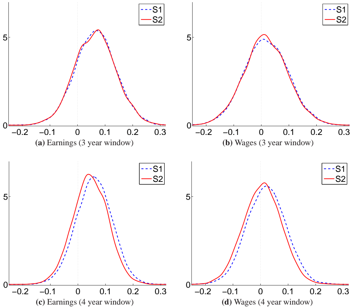
Figure 3: Kernel-smoothed densities of the posterior density of RDDCATE for the preferred specifications 1 and 2 (under 5 degrees of freedom) for earnings and wages.
