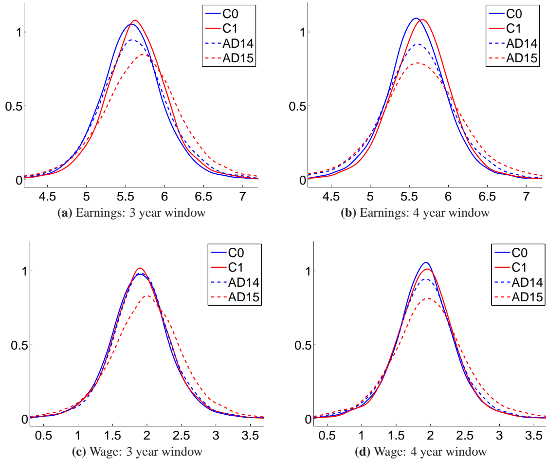
Figure 2: Kernel-smoothed predictive densities of potential earnings and wage by type and treatment for the preferred model.
