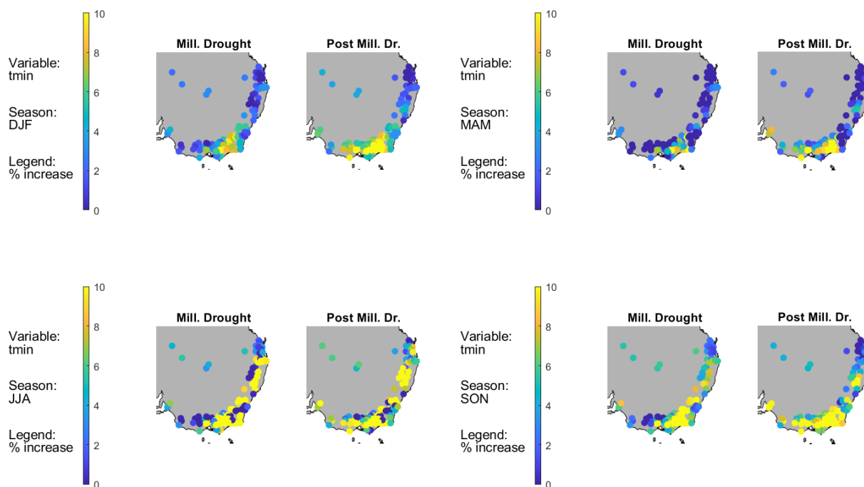
Figure D6. Same as Fig. D1 except for t_{\min} (minimum daily temperature). Based on data from Fowler et al. (2021).
