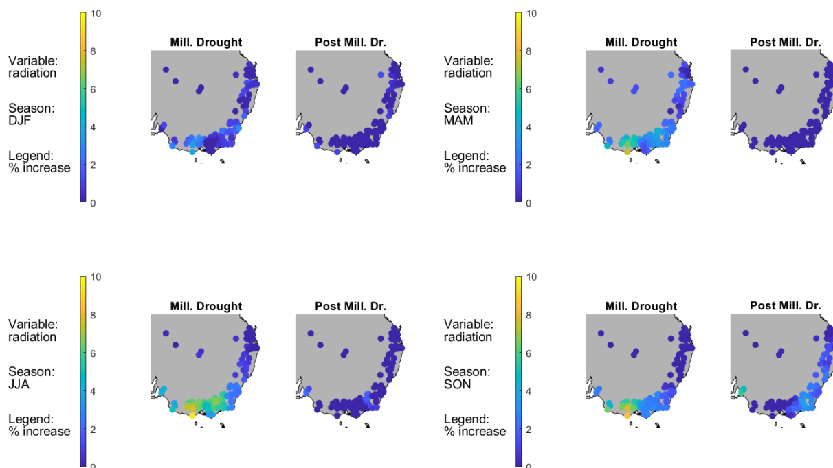
Figure D5. Same as Fig. D1 except for radiation. Based on data from Fowler et al. (2021).
