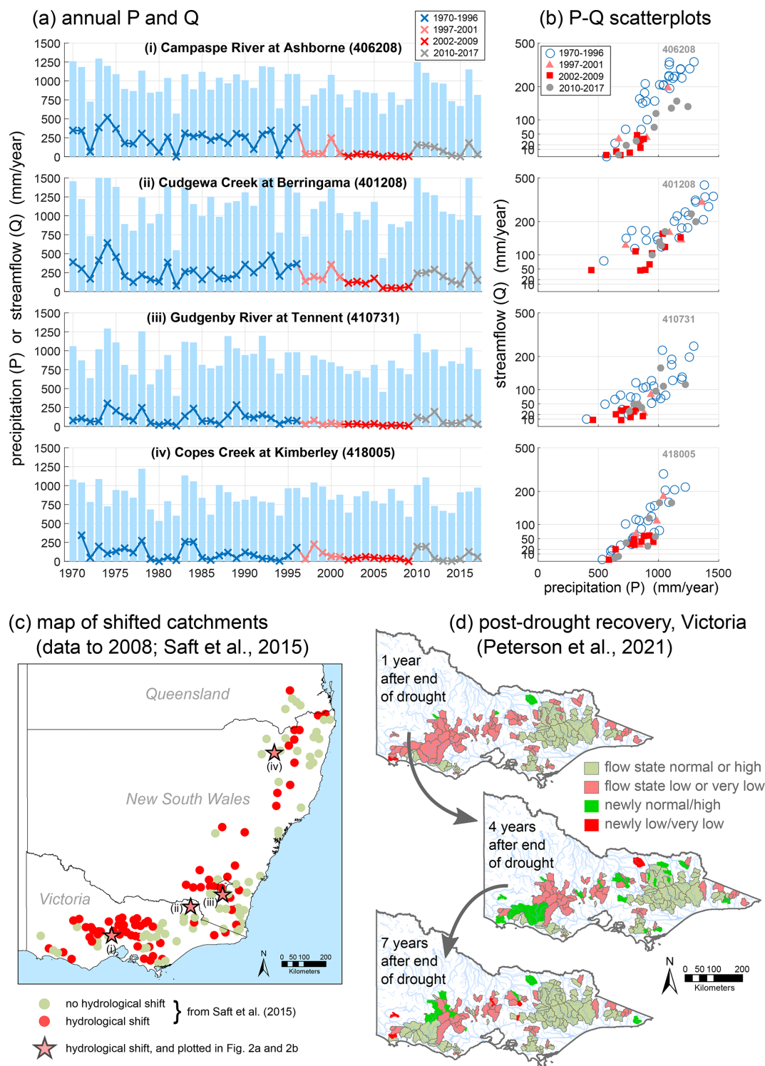
Figure 2. Hydrological behaviour prior to and during the Millennium Drought (a–c) and post-drought recovery (d), based on prior studies. (a) annual time series of precipitation ( P ; bars) and streamflow ( Q ; lines and crosses) for four selected catchments which exhibited hydrological shifts. (b) Scatterplots corresponding to panel (a). (c) Location map of shifted catchments from Saft et al. (2015). (d) Drought recovery with time and mapped across the state of Victoria for selected time slices from Peterson et al. (2021). Elapsed time is measured from the end of the meteorological drought.
