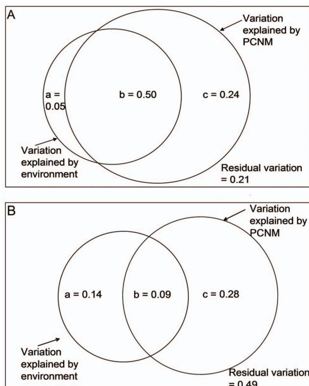
Figure 2. Variation partitioning results. Venn diagrams represent the partitioning variation in the archaeal community (beta-diversity) in different habitats (A) non-flooded soil (NS) and (B) flooded soil (FS). Each box represented 100% of the variation in the corresponding response variable, and the reported fractions were adjusted R^2 statistics ( R^2 ). doi:10.1371/journal.pone.0063375.g002
