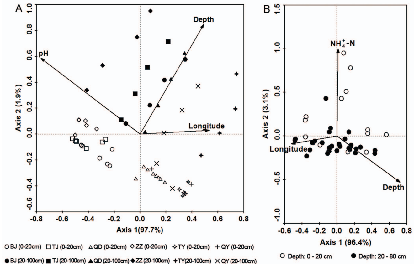
Figure 3. Redundancy analysis (RDA) for the relationship between environmental or geographic variables and archaeal community composition. (A) non-flooded soil (NS) and (B) flooded soil (FS).
