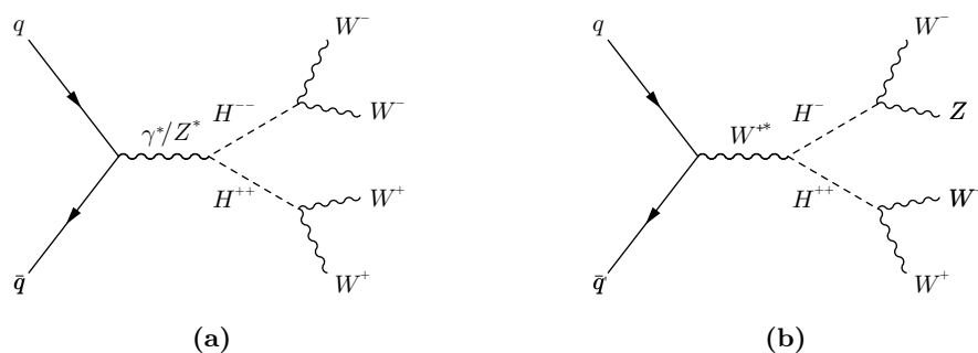
Figure 1. Feynman diagrams illustrating production and subsequent decay of the H^{\pm\pm} and H^{\pm} bosons: (a) H^{\pm\pm} pair production and (b) H^{\pm\pm} and H^{\pm} associated production.
