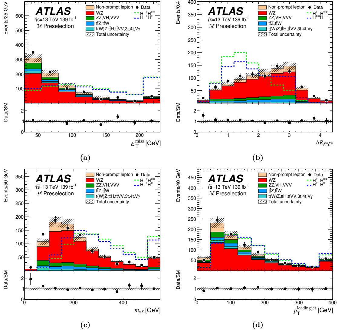
Figure 4. Distribution of selected variables used to define the 3\ell SRs. The events are selected with the preselection requirements listed in table 4. The data (dots) are compared with the expected contributions from the relevant background sources (histograms). The expected signal distributions for m_{H^{\pm\pm}} = 300 GeV are also shown, scaled to the observed number of events. The last bin includes overflows. In each figure the bottom panel shows the ratio of data to the estimated background. The hatched band around unity represents the total uncertainty of the background.
