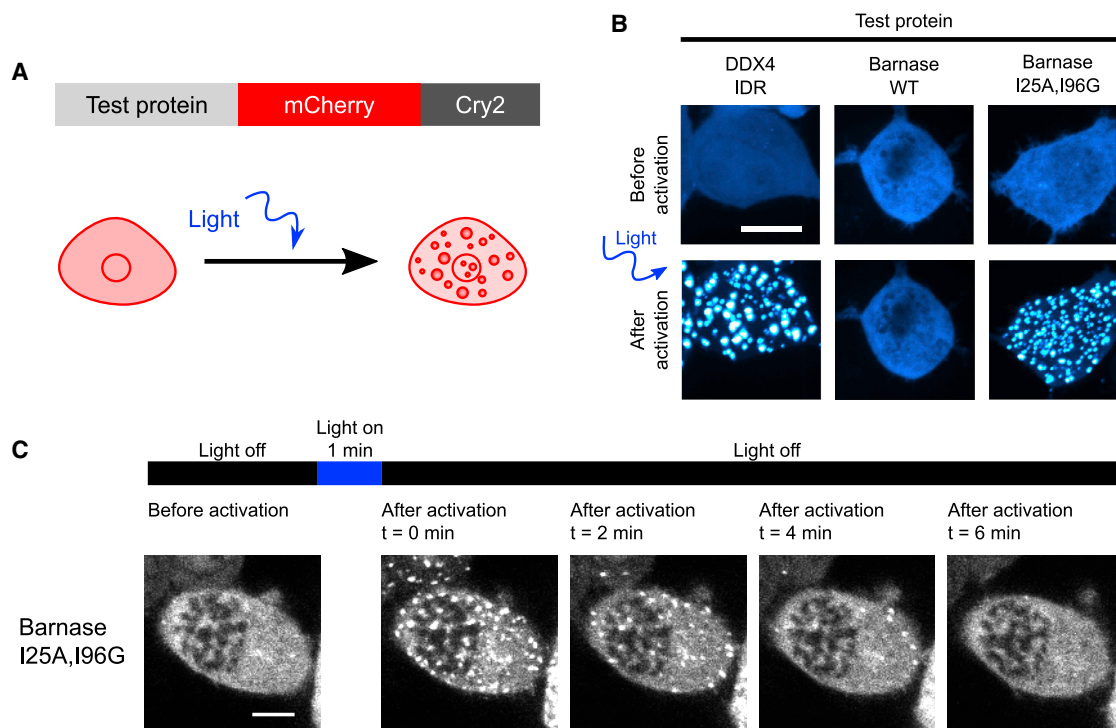
Figure 2. Phase separation is driven by interactions among unfolded barnase molecules
