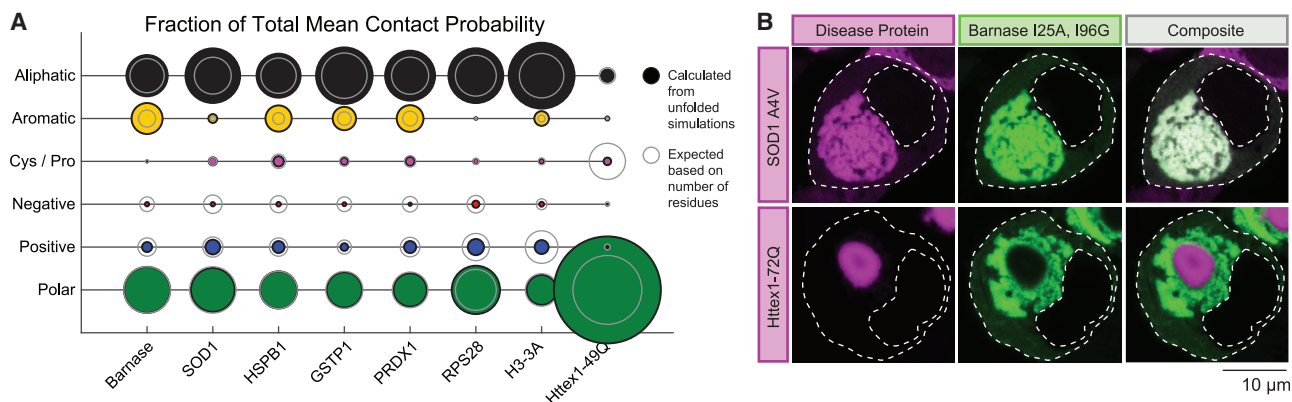
Figure 7. Sequence grammar that drives the phase separation of unfolded states is similar between barnase and disease-associated IFPs (A) Fraction of total mean contact probability per residue type calculated from atomistic simulations of the unfolded state (STAR Methods). (B) Fluorescence micrographs show deposits formed by a destabilized variant of barnase (I25A, I96G) flanked with fluorescent proteins (mTFP1 and Venus) (Wood et al., 2018) along with deposits formed by mutant SOD1 (SOD1 A4V) or mutant Httex1 containing a glutamine tract of 72 residues fused to mCherry. The constructs were co-transfected in HEK293T cells. Outlines of cells and nuclei are shown with dashed lines.
