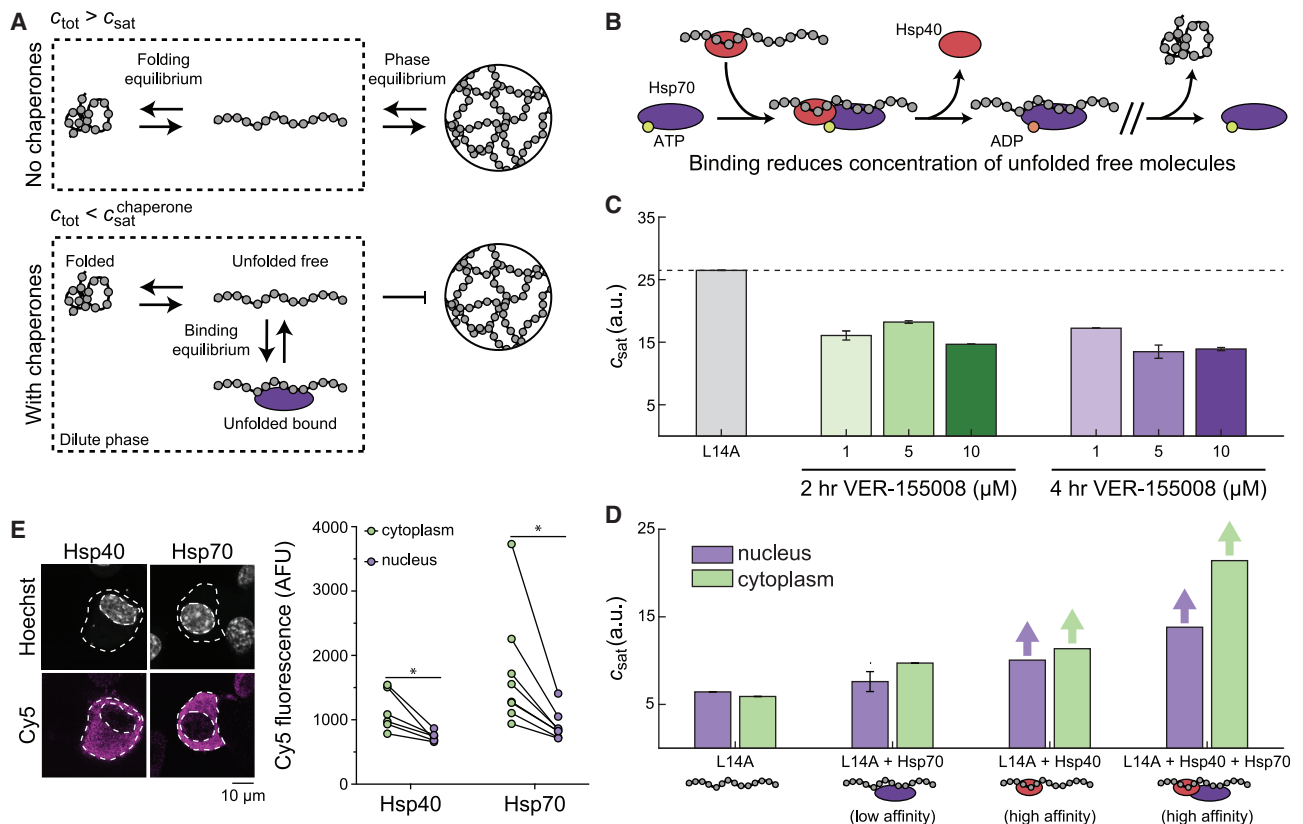
Figure 5. Molecular chaperones suppress phase separation
