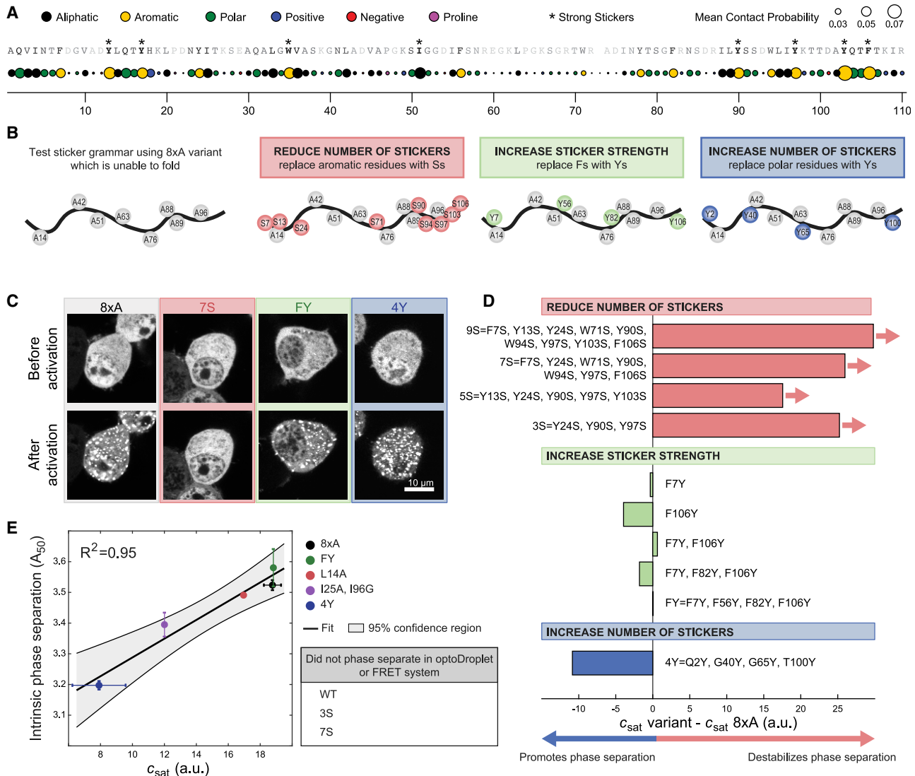
Figure 4. Phe and Tyr function as stickers that drive the phase separation of unfolded barnase
