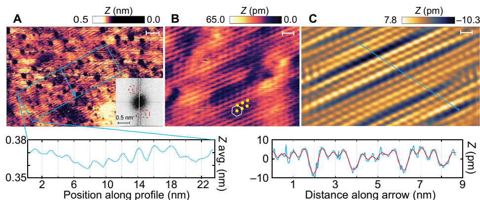
Fig. 5. STM measurements. (A) Large-area STM image of \beta' - \text{In}_2\text{Se}_3 at 77 K. Scale bar, 10 nm. The bottom graph presents the height profile of 1D superstructures, and the inset indicates the fast Fourier transform pattern showing spots of the superstructures. (B) Zoomed-in STM image showing the atomic structure of unit cell and the 1D superstructures due to height modulation. Scale bar, 1 nm. (C) Atomic structure of 1D superstructures taken from another region. The bottom graph shows the height profile taken from the blue line. Scale bar, 1 nm.
