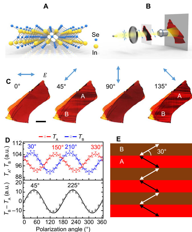
Fig. 1. Linear dichroism of \text{In}_2\text{Se}_3 . (A) Crystal structure of layered \beta\text{-In}_2\text{Se}_3 . (B) Schematic of the linear polarization optical microscopy measurement. (C) Optical image sequence of \beta\text{-In}_2\text{Se}_3 imaged by light of different polarization angles. Scale bar, 25 \mu\text{m} . (D) Polarization angle dependence of the light transmission of the regions A and B as shown in (C). a.u., arbitrary units. (E) Schematic of the optical axes of regions A and B.
