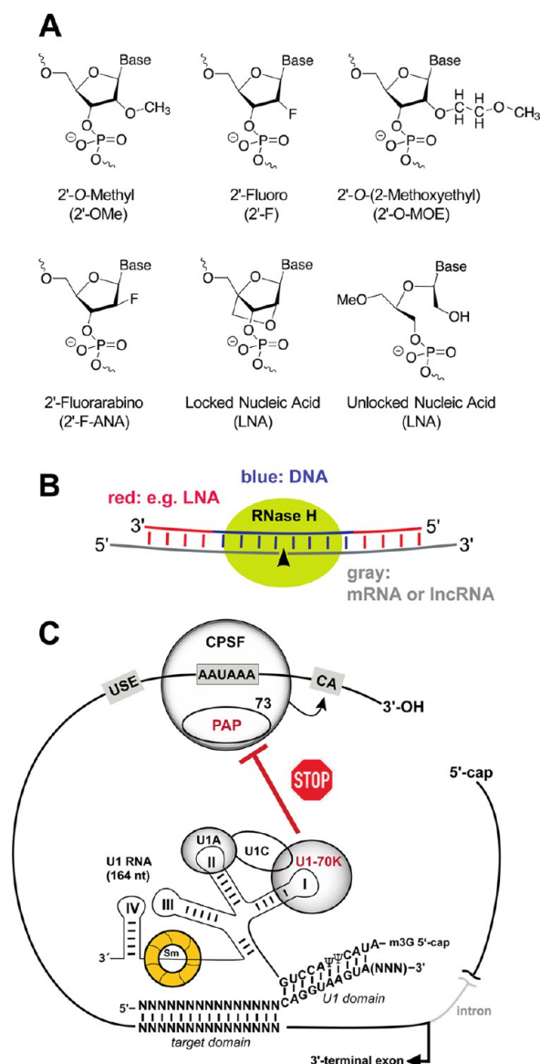
Figure 26. (A) Chemical nucleoside modifications frequently used for nucleic acid effectors. In many cases, phosphorothioate (PS) modifications (one of the two nonbridging oxygens of the phosphodiester replaced with sulfur) are incorporated, to improve the pharmacokinetic properties and cellular uptake. (B) LNA gapmers composed of terminal LNA residues and at least 6 central DNA nucleotides enable cleavage of RNA target strands as part of RNA:DNA hybrids by endogenous RNase H activities. (C) In the U1 adaptor approach, a U1 small nuclear ribonucleoprotein (snRNP) (an abundant spliceosomal RNP) is guided to the 3'-terminal exon of a target pre-mRNA via a dual antisense oligonucleotide that simultaneously anneals to the 5'-end of U1 RNA. This blocks polyadenylation via an inhibitory interaction between poly(A) polymerase (PAP) and the U1-70K protein. As a result, the pre-mRNA is still cleaved but not polyadenylated, which induces its degradation. Efficient down-regulation by “U1 interference (U1i)” was observed with target domains of 12–15 nt (with up to 15 LNA residues) and 10–13 nt in the U1 RNA binding domain (good efficiency observed with eight 2'-O-methyl and five LNA residues). A PS backbone was also found to be compatible with U1i. 499,500 U1A, U1C, U1-70k and the Sm ring proteins are integral components of the U1 snRNP. PAP: poly(A) polymerase; CPSF: cleavage and polyadenylation specificity factor (including the endonucleolytic subunit 73); CA: cleavage site. Adapted with permission from ref 500. Copyright 2009 John Wiley & Sons, Inc.
