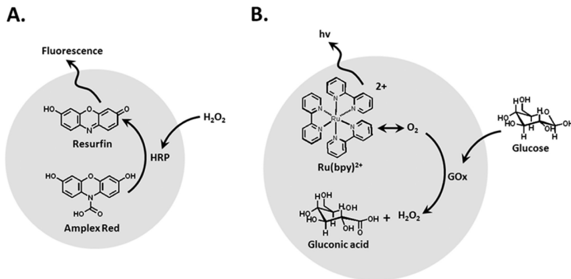
Figure 16. Bifunctional recognition/dye polymer NPs for sensing: (A) Sensing of H_2O_2 via the HRP-driven oxidation of Amplex-Red to the fluorescent Resorufin product. (B) Sensing of glucose by the depletion of O_2 by the GOx-mediated oxidation of glucose, using Ru(bpy)_3^{2+} as auxiliary fluorescent probe.
