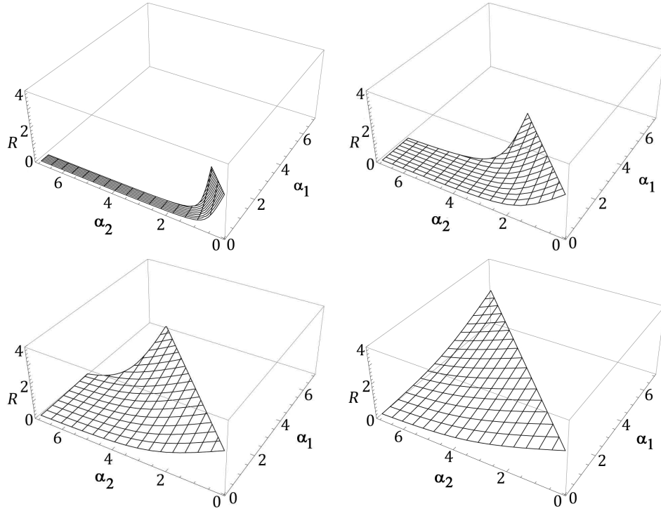
Figure 6: The plots of R as a function of the lethalitys ( \alpha_1, \alpha_2 ), in the same four cases as on Figs. 3, 4: \lambda = 2, 6, 10 and 14 (from left to right, top to bottom), when all the other parameters of the model are common ( \beta_1 = 0.3, \beta_2 = 0.6, \mu_1 = \mu_2 = 0.2 ). The plots are restricted to the regions where the respective processes are supercritical and \alpha_1 < \alpha_2 (as we assumed). Note the unusual orientation of the \alpha -coordinate axes (chosen so as to have a better view of the plots).
