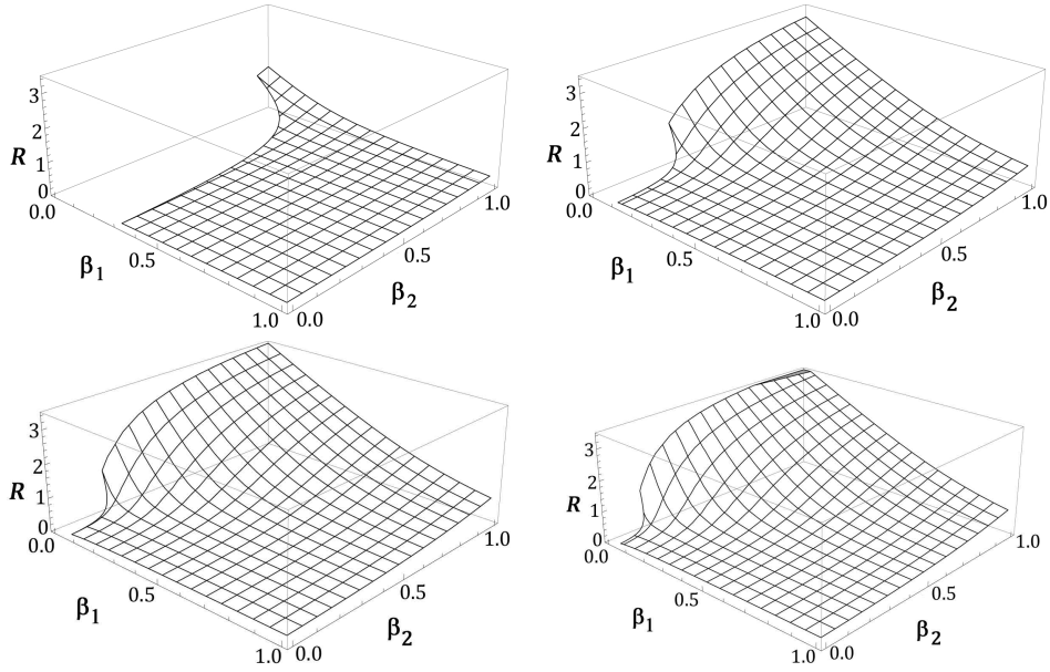
Figure 4: The plots of the limiting value R as a function of the transmissibility probabilities (\beta_1, \beta_2) in four cases: \lambda = 2, 6, 10 and 14 (from left to right, top to bottom), when all the other parameters of the model are common ( \alpha_1 = 0.5 , \alpha_2 = 1.5 , \mu_1 = \mu_2 = 0.2 ). The plots are restricted to the regions where the respective processes are supercritical.
