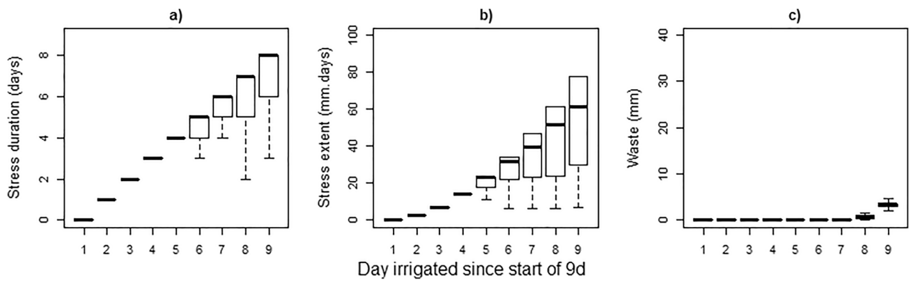
Fig. 5 The ensemble simulations of: a) stress duration in days; b) stress extent in mm.day, and c) waste extent in mm. All risks are plotted for different irrigation timing decisions i.e., to water on Day 1–9 within the future 9 days starting on Day 42 in the season (x-axes). All boxplots are shown with no outliers and whiskers are 1.5 times the interquartile ranges
