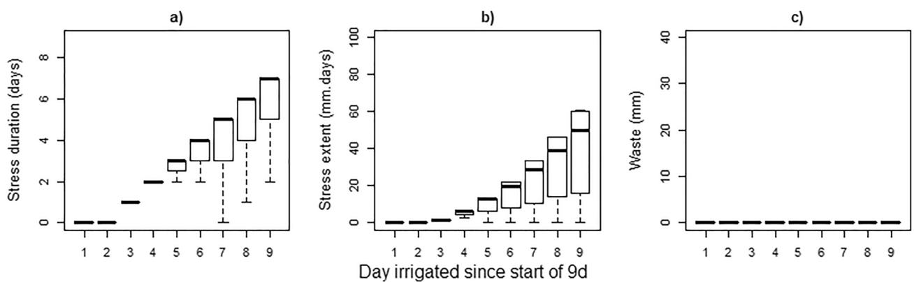
Fig. 7 The ensemble simulations of: a) stress duration in days; b) stress extent in mm.day, and c) waste extent in mm. All risks are plotted for different irrigation decisions i.e., to water on Days 1–9 within the future 9 days starting on Day 66 in the season (x-axes). All boxplots are shown with no outliers and whiskers are 1.5 times the interquartile ranges
