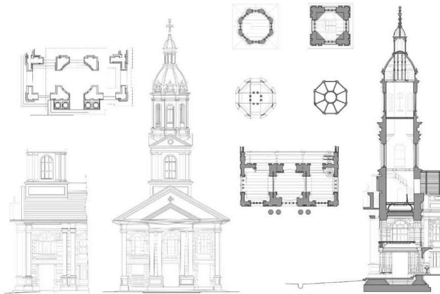
Fig. 2. Amended plans for the Church of the Sacred Heart on Tank Road designed by Tomlinson and Lermi, 1908. Redrawn by Chen Jingwen.
