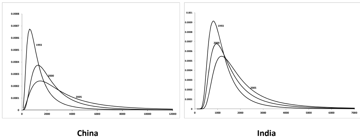
Figure 2: Density Functions over Time, China and India
