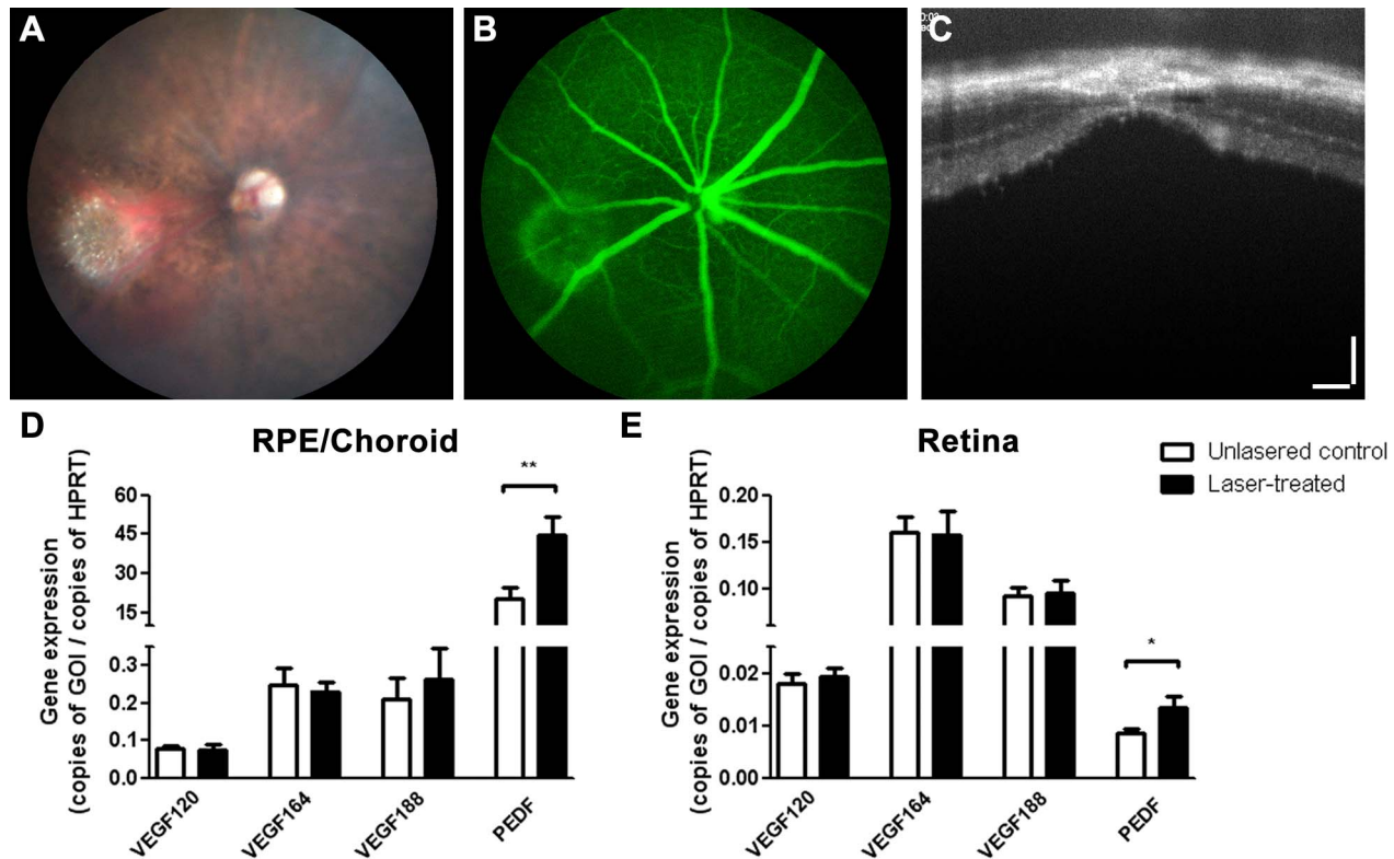
FIGURE 8. Suprathreshold nanosecond laser treatment causes a fundus lesion and retinal neuronal loss but little change in angiogenic gene expression in the RPE and retina in mice. C57BL/6J mice were treated with suprathreshold nanosecond laser (0.5 mJ). (A) At 7 days, the retinal fundus was imaged with the Micron III fundus-OCT system. Color fundus imaging showed suprathreshold laser treatment induced a large white lesion. (B) Fluorescein angiography showed fluorescence leakage around the edges of the lesion site. (C) OCT imaging showed a loss of retinal neurons and a large hyperfluorescent lesion suggestive of scarring in the center of the laser site. (D, E) To determine if the suprathreshold laser dose induced gene expression changes consistent with neovascularization, the retina and RPE were isolated separately for analysis of VegfA isoforms ( VegfA120 , VegfA164 , VegfA188 ) and Pedf relative to the housekeeping gene Hprt . Unlasered C57BL/6J mice tissues were used as controls. (D) In laser-treated RPE samples, expression of VegfA 120 , 164 , and 188 isoforms were not altered, while Pedf mRNA expression was upregulated when compared with unlasered controls (* P < 0.05). (E) Similarly, in laser-treated retinal samples, expression of VegfA 120 , 164 , and 188 isoforms were not altered, while Pedf mRNA expression was upregulated (** P < 0.01). Data are presented as mean ± SEM for at least n = 9 mice per group. Scale for (C): vertical, 100 μm; horizontal, 100 μm.
