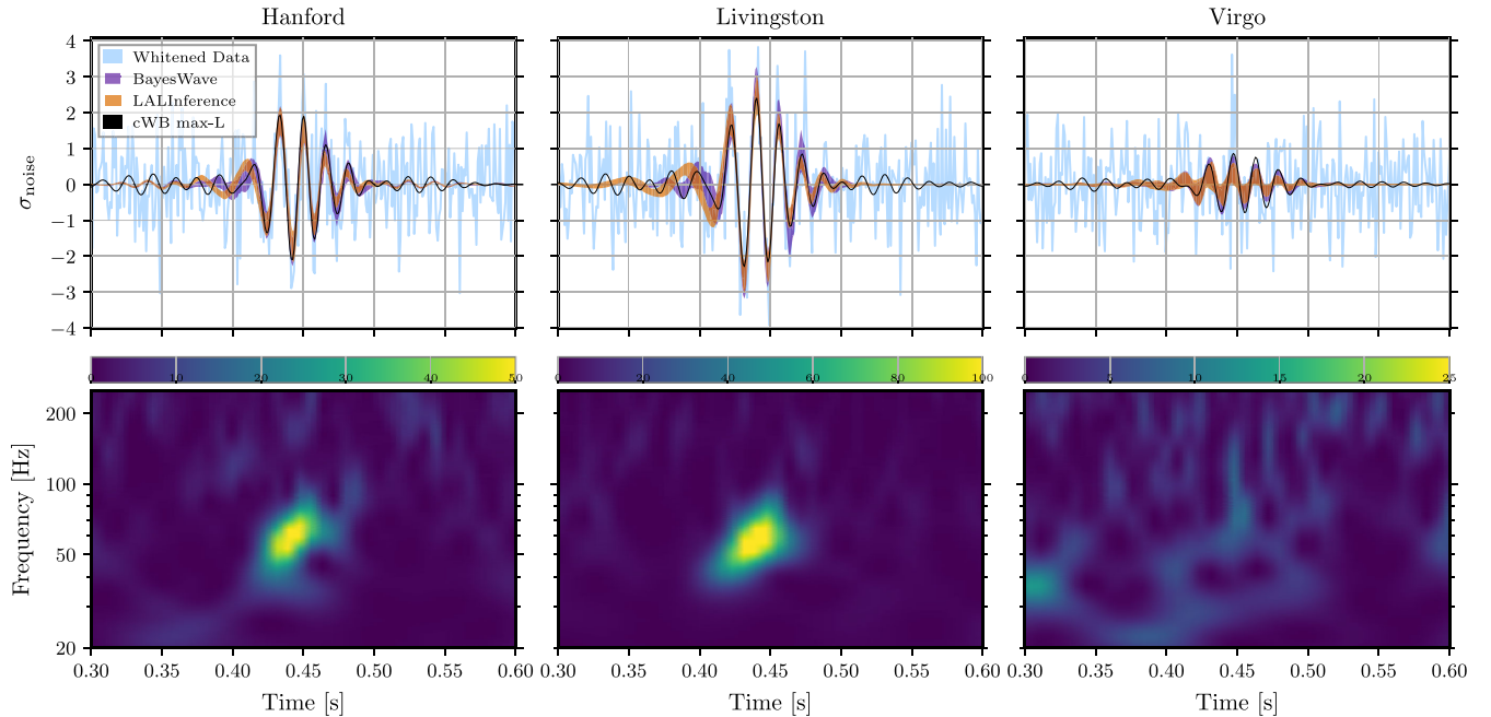
FIG. 1. The GW event GW190521 observed by the LIGO Hanford (left), LIGO Livingston (middle), and Virgo (right) detectors. Times are shown relative to May 21, 2019 at 03:02:29 UTC. The top row displays the time-domain detector data after whitening by each instrument's noise amplitude spectral density (light blue lines); the point estimate waveform from the CWB search [43] (black lines); the 90% credible intervals from the posterior probability density functions of the waveform time series, obtained via Bayesian inference (LALInference [49]) with the NRSur7dq4 binary BH waveform model [50] (orange bands), and with a generic wavelet model (BayesWave [51], purple bands). The ordinate axes are in units of noise standard deviations. The bottom row displays the time-frequency representation of the whitened data using the Q transform [52].
