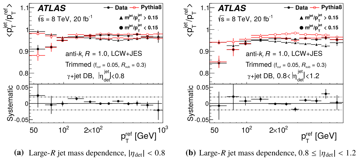
Fig. 30 R_{\text{DB}} as a function of p_{\text{T}}^{\text{ref}} measured for trimmed anti- k_t jets with R = 1.0 in \gamma +jet events shown separately for jets with a |\eta_{\text{det}}| < 0.8 and b 0.8 \leq |\eta_{\text{det}}| < 1.2 . Separate results are shown for jets with m/p_{\text{T}} < 0.15 and m/p_{\text{T}} > 0.15 , displayed with circles and triangles, respectively. Measurements in data are shown as filled
