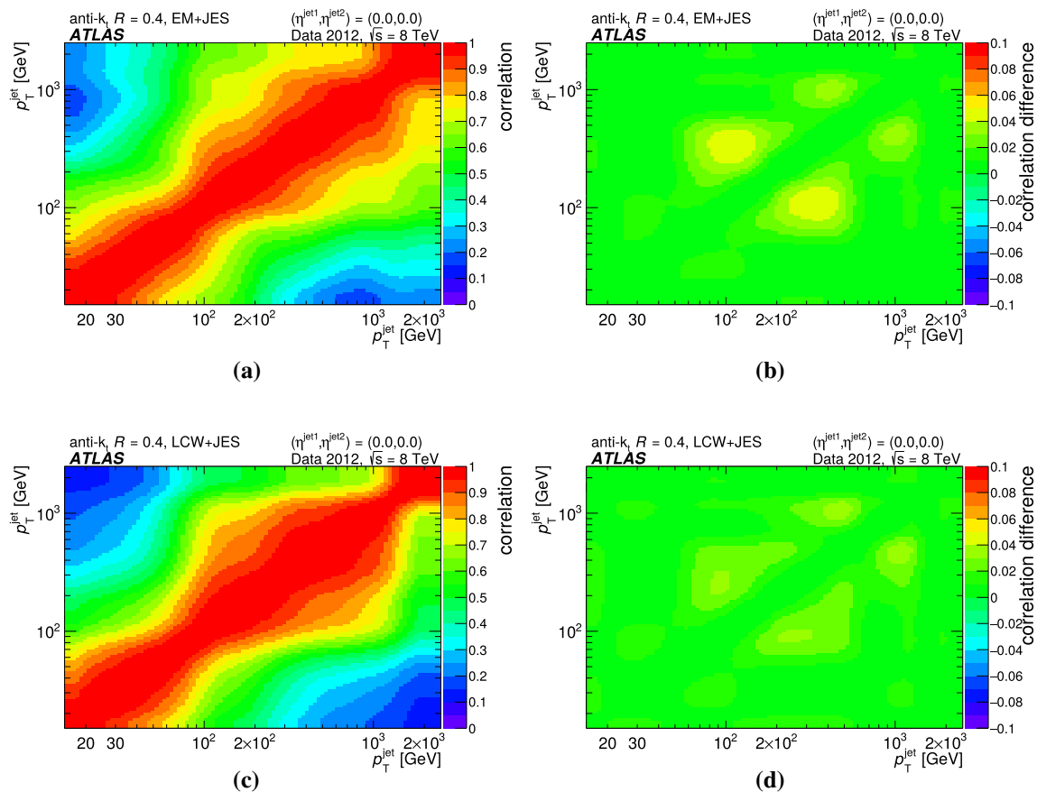
Fig. 45 The a , c JES correlation matrix and b , d difference between the full correlation matrix and that derived from a reduced number (6) of absolute in situ uncertainty components for anti- k_T , R = 0.4 jets calibrated with the a , b EM+JES and c , d LCW+JES schemes
