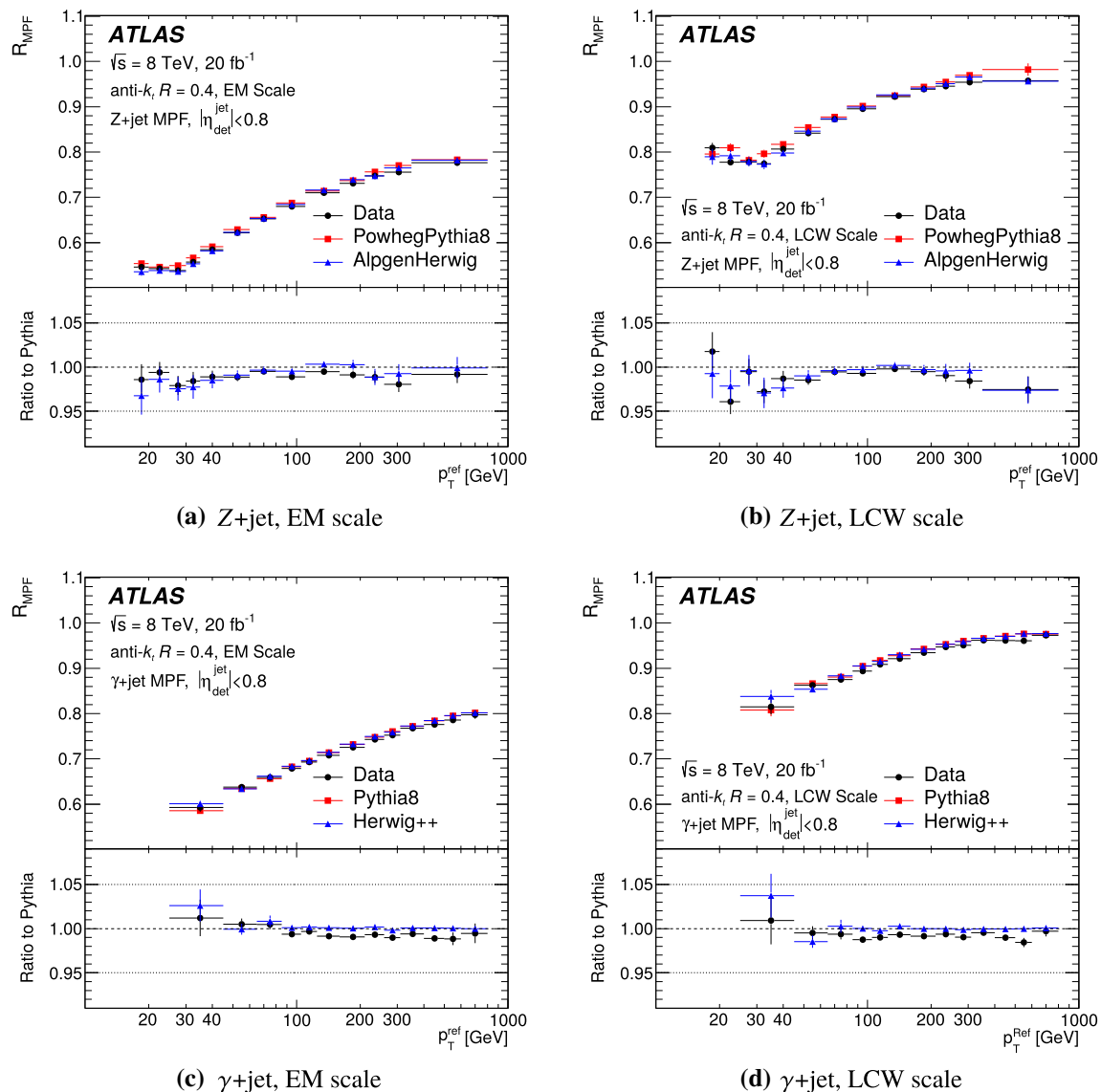
Fig. 24 The MPF response R_{\text{MPF}} in a , b Z+jet and c , d \gamma +jet events for jets calibrated a , c at the EM scale and b , d using the LCW scheme, for both data and MC simulation, as a function of p_T^{\text{ref}} . Only statistical uncertainties are shown
