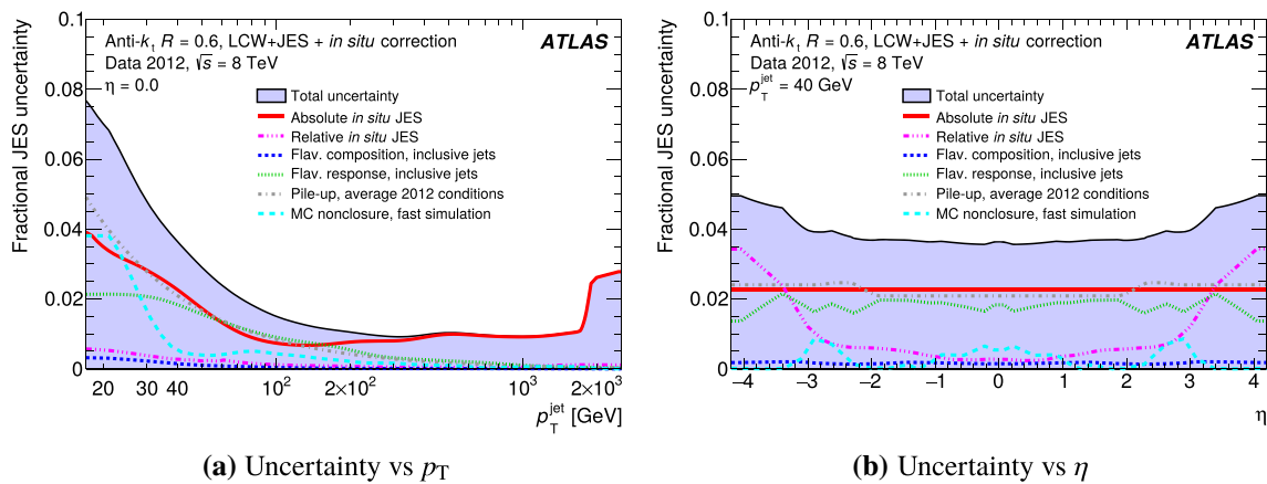
Fig. 44 Total uncertainty in the calibration of anti- k_T , R = 0.6 jets in fast simulation as a function of p_T and \eta . The large “MC non-closure” term demonstrates the limitations of using R = 0.6 jets in fast sim-
