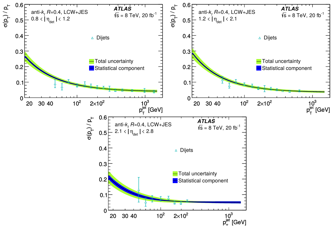
Fig. 58 The jet resolution as a function of p_T for LCW+JES anti- k_T R = 0.4 jets in three more-forward regions. The dijet in situ inputs (empty triangles) to the measurement are shown. The final fit using the function in Eq. (24) is included with its associated statistical and total uncertainty
