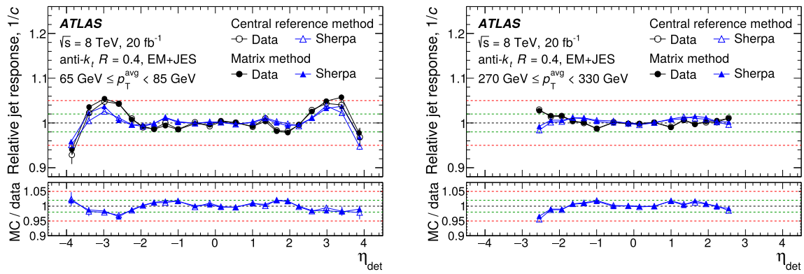
Fig. 16 Relative jet response measured using the matrix and central reference methods for anti- k_t jets with R = 0.4 calibrated with the EM+JES scheme as a function of the probe jet pseudorapidity. Results are presented for 65 \text{ GeV} \leq p_T^{\text{avg}} < 85 \text{ GeV} and 270 \text{ GeV} \leq p_T^{\text{avg}} < 330 \text{ GeV}
