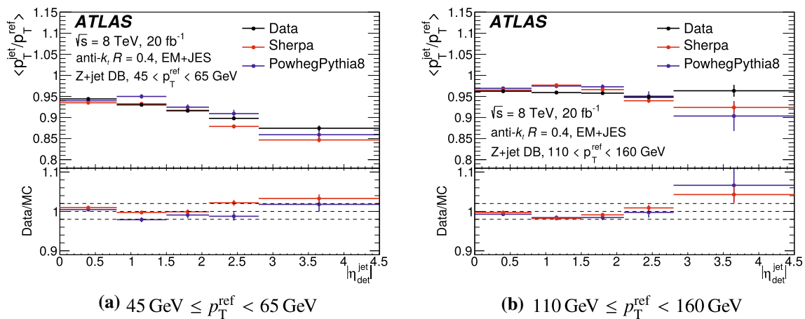
Fig. 23 R_{DB} as a function of \eta_{det} for anti- k_t jets with R = 0.4 calibrated with the EM+JES scheme in data (black), as well as in SHERPA (red) and POWHEG+PYTHIA8 (blue) simulation, for a 45 \text{ GeV} \leq p_T^{ref} < 65 \text{ GeV} and b 110 \text{ GeV} \leq p_T^{ref} < 160 \text{ GeV} . Only statistical uncertainties are shown
