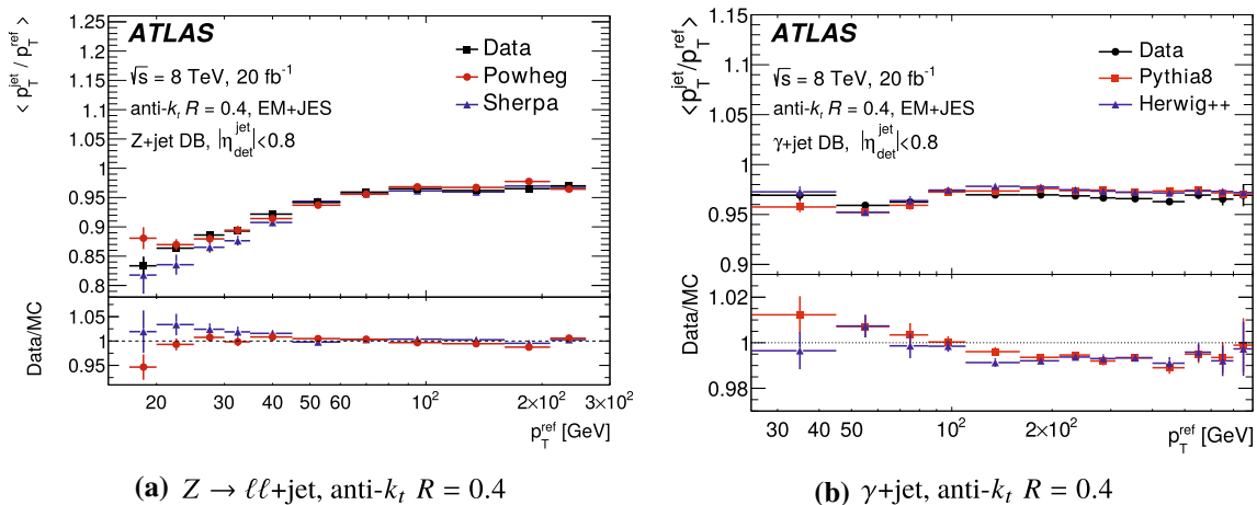
Fig. 22 R_{\text{DB}} for anti- k_t jets with R = 0.4 and calibrated with the EM+JES scheme from the a Z+jet and b \gamma +jet analyses in the data and for two MC simulations. Only statistical uncertainties are shown
