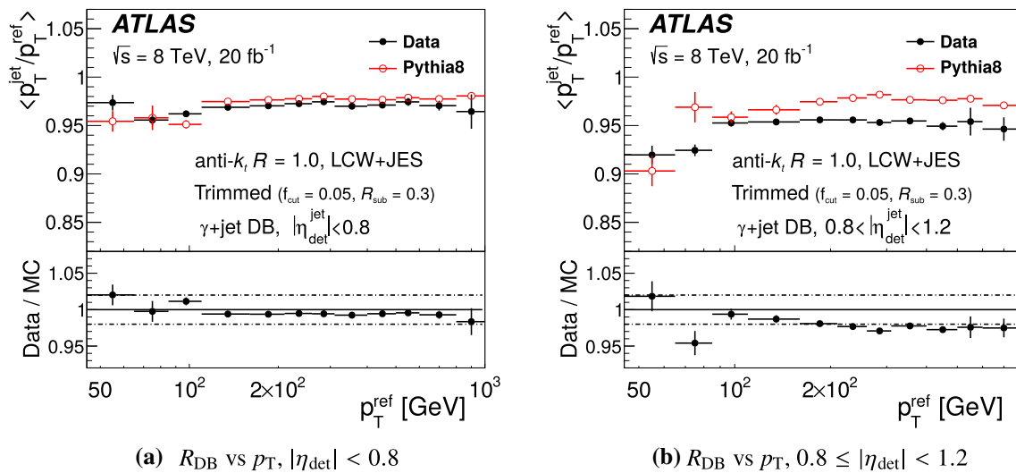
Fig. 29 R_{\text{DB}} for trimmed anti- k_t jets with R = 1.0 calibrated with the LCW+JES scheme for a |\eta_{\text{det}}| < 0.8 and b 0.8 \leq |\eta_{\text{det}}| < 1.2 for both data (filled circles) and MC simulation (empty circles), as a function of the p_T^{\text{ref}} . Only statistical uncertainties are shown
