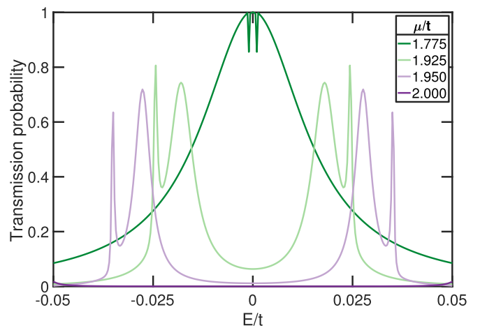
FIG. 5. Transmission probability of an AB ring at energies about zero for several different values of the on-site potential \mu . The AB ring has a p -wave pairing amplitude \Delta/t = 1.0 and normal leads are attached with a coupling strength of \tau/t = 0.3 . The external applied magnetic field strength here is \Phi/\Phi_0 = 0 .
