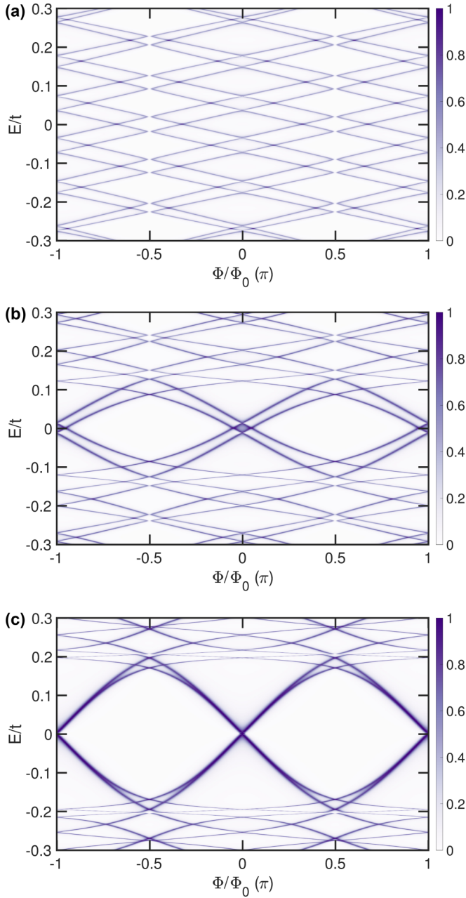
FIG. 7. Transmission probability of an AB ring as a function magnetic flux \Phi and energy E for various values of p -wave pairing amplitude (a) \Delta/t = 0 , (b) \Delta/t = 0.05 , and (c) \Delta/t = 0.1 . The AB ring has an on-site potential \mu/t = 1.0 and normal leads are attached with a coupling strength of \tau/t = 0.3 .
