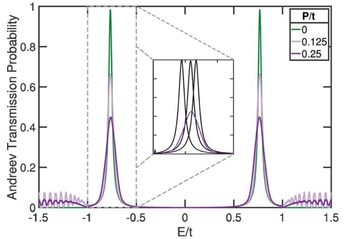
FIG. 10. Transmission in an AB ring with \Delta/t = \mu/t = 1.0 , 50 sites and a magnetic field of \phi/\phi_0 = \frac{\pi}{2} , for several values of disorder strength P . Each disorder value in this figure has been averaged over 1000 configurations. The inset shows a sample of the static disorder realisations together with the dynamic disorder result for a disorder strength of P/t = 0.25 .
