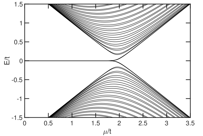
FIG. 4. Eigenenergies for an AB ring (without leads attached) as a function of \mu/t with \Delta/t = 1.0 . Here the magnetic flux through the ring is \Phi/\Phi_0 = 0 .
