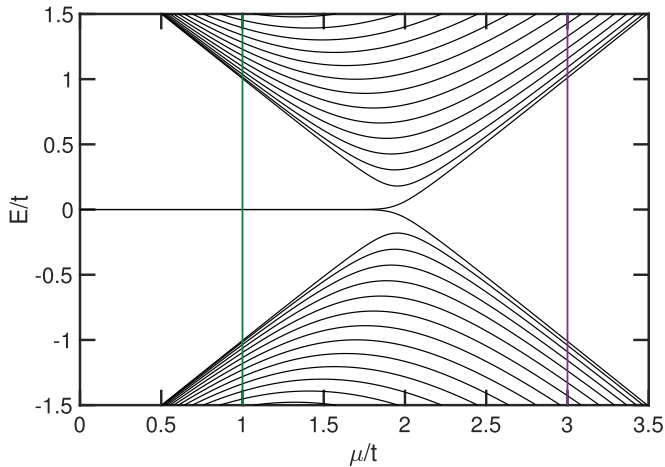
FIG. 2. Eigenenergies for a 1D Kitaev nanowire as a function of \mu/t with \Delta/t = 1.0 . Vertical lines indicate values of \mu/t used to compute the transmission probabilities in Fig. 3.
