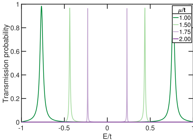
FIG. 9. Transmission probability of an AB ring with 50 \times 2 sites as a function of energy E for various on-site potentials \mu and a magnetic flux of \Phi/\Phi_0 = \frac{\pi}{2} . The AB ring has a p -wave pairing amplitude \Delta/t = 1.0 and normal leads are attached with a coupling strength of \tau/t = 0.3 . When \mu/t = 2 the transmission is zero for all energies.
