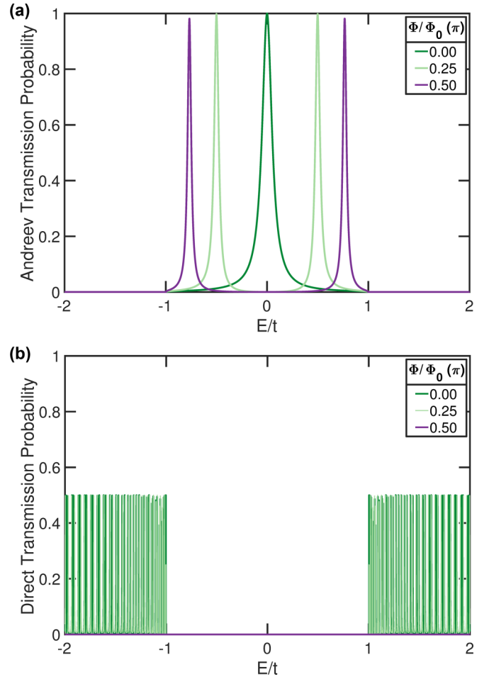
FIG. 8. Contributions to the transport probability from (a) Andreev and (b) direct transmission for an AB ring with 50 \times 2 sites as a function of energy E . Here the on-site potential is \mu/t = 1 . The AB ring has a p -wave pairing amplitude \Delta/t = 1.0 and normal leads are attached with a coupling strength of \tau/t = 0.3 .
