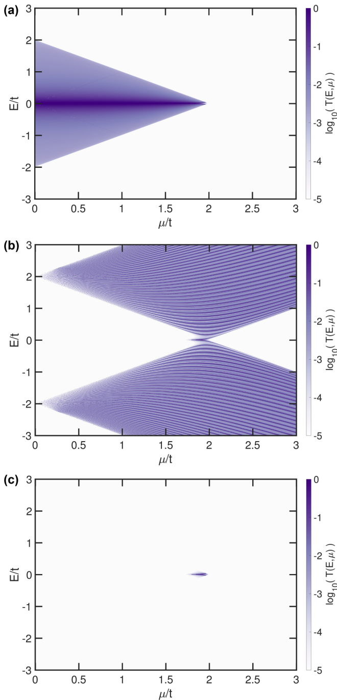
FIG. 6. Contributions to the transmission probability from (a) Andreev, (b) direct, and (c) crossed Andreev transmission for an AB ring with 50 \times 2 sites as a function of energy E and on-site potential \mu . Here the magnetic flux through the ring is \Phi/\Phi_0 = 0 . The AB ring has a p -wave pairing amplitude \Delta/t = 1.0 and normal leads are attached with a coupling strength of \tau/t = 0.3 . Note the logarithmic color scale used in order to resolve the weaker transmission probabilities in (b) and (c).
