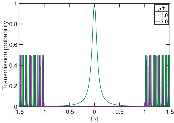
FIG. 3. Transmission probability as a function of energy for the 1D Kitaev nanowire for two values of \mu/t , highlighted in Fig. 2 as vertical lines. The nanowire has a p -wave pairing amplitude of \Delta/t = 1.0 and a hopping strength between the leads and the device of \tau/t = 0.3 .
