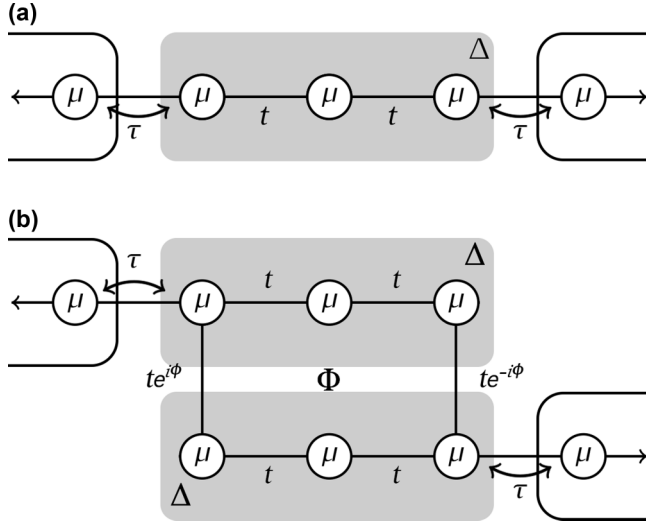
FIG. 1. A diagram of a 1D Kitaev nanowire (a) and Aharonov-Bohm ring (b). These consist of a tight binding chain with onsite potential \mu , hopping strength t , and a p -wave pairing amplitude of \Delta . Normal leads are coupled to the nanowire with a hopping amplitude of \tau .
