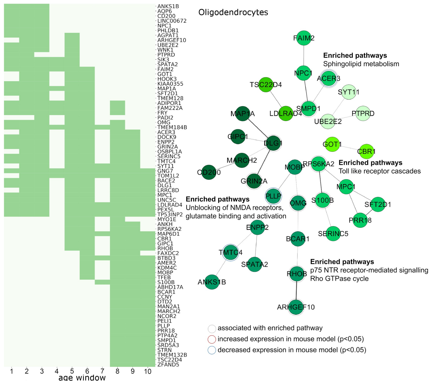
Fig 6. Cellular pathways associated with genes expressed by oligodendrocytes and developmental alterations in the preterm cortex. Left: Genes expressed by oligodendrocytes in the fetal cortex and significantly associated with group differences in T1w/T2w contrasts across at least 3 age windows are shown. Dark green indicates periods where gene expression and T1w/T2w contrast were significantly correlated for each gene (FDR p < 0.05 ) across the preterm period. Right: PPI networks derived using STRING. Top functional enrichments of molecular pathways are shown where applicable. Genes associated with listed enriched pathway and genes differentially expressed in an animal model of preterm brain injury are highlighted. See https://github.com/garedaba/baby-brains/tree/master/data/gene_lists . FDR, false discovery rate; PPI, protein-protein interaction; STRING, Search Tool for the Retrieval of Interacting Genes/Proteins.
