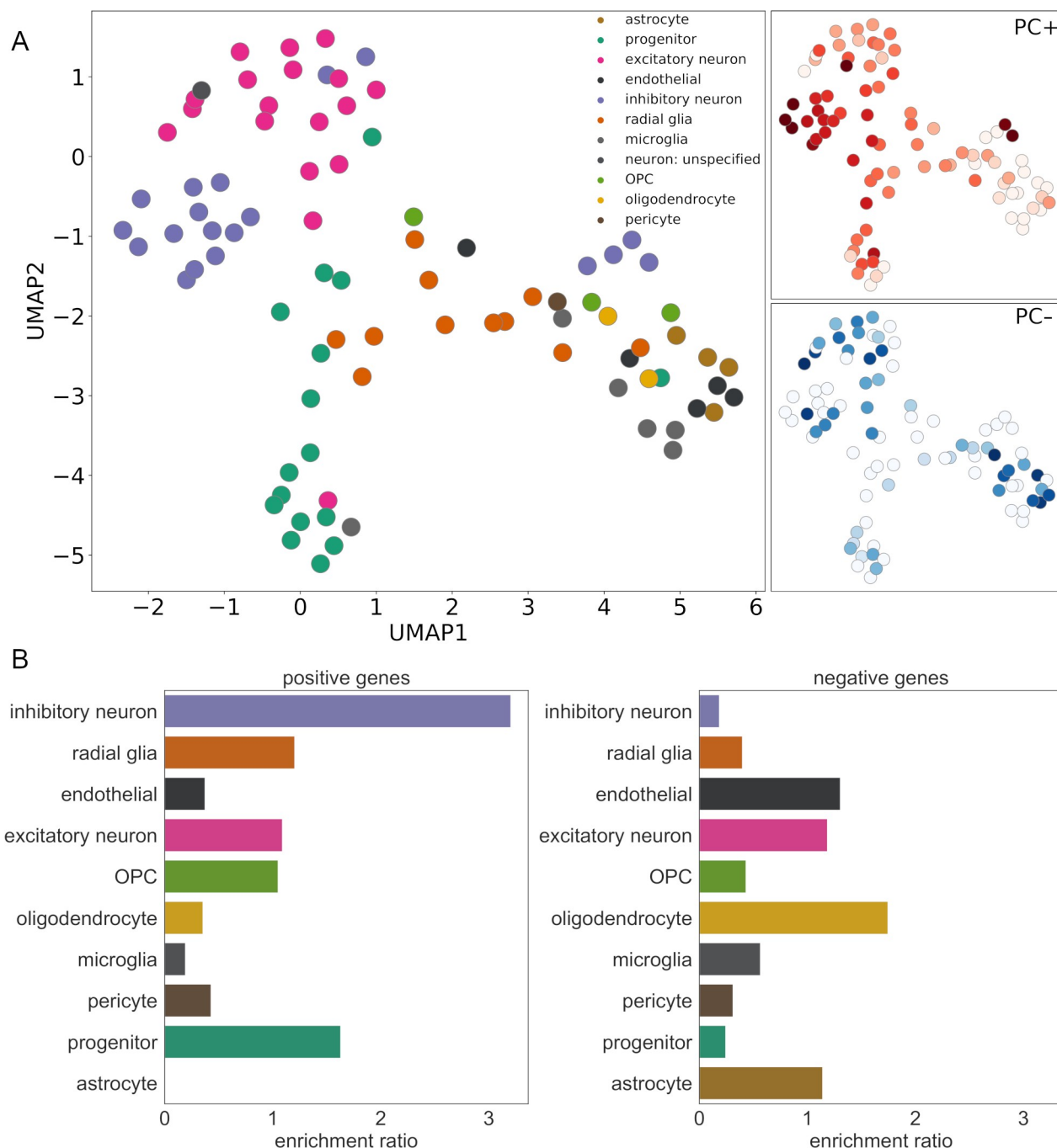
Fig 3. Cell-specific gene expression is associated with cortical morphology at birth. (A) UMAP embedding of 86 cell types based on trajectories of relative gene expression over time recovers annotated cell classes. Subplots reflect enrichment ratios of cell classes in PC+ and PC- gene sets (darker colour represents higher enrichment ratio). (B) Enrichment ratio for fetal marker genes expressed by each cell class is shown for PC+ (left) and PC- (right) gene sets. See https://github.com/garedaba/baby-brains/tree/master/figures . OPC, oligodendrocyte precursor cell; UMAP, Uniform Manifold Approximation and Projection.
