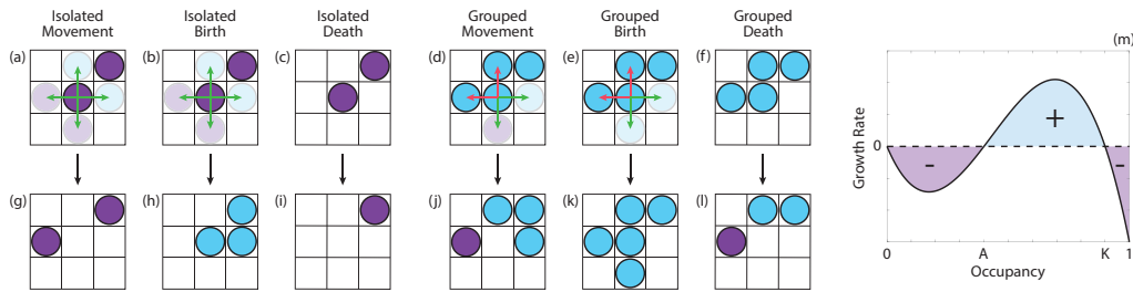
Figure 2. Mechanisms in the Allee random walk model. (a)-(c) Potential movement, birth and death events, respectively, for the isolated individual in the centre of the lattice. (d)-(f) Potential movement, birth and death events, respectively, for the grouped individual in the centre of the lattice. Green arrows indicate directions that would result in a successful event, red arrows indicate directions that would result in an unsuccessful event. (g)-(l) Lattice configuration after the corresponding event in (a)-(f). Isolated individuals are shown in purple, grouped individuals are shown in cyan. (m) Typical growth rate curve as a function of the occupancy of the lattice. Cyan regions correspond to positive growth and purple regions correspond to negative growth. A is the threshold parameter and K is the carrying capacity.
