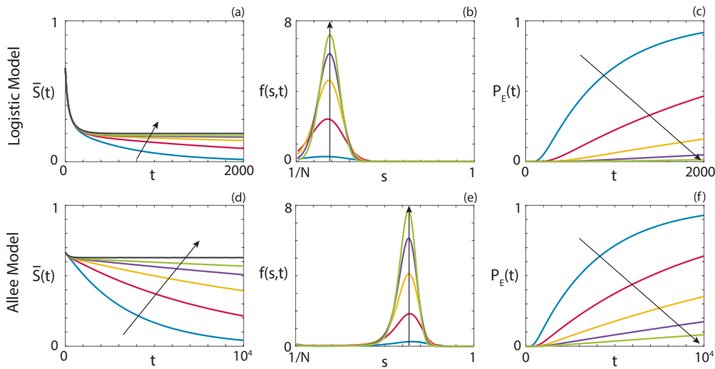
Figure 7. SSDA predictions for the (a),(d) the evolution of the average occupancy, (b),(e) the occupancy distribution probability density function, and (c),(f) the evolution of the extinction probability for (a)-(c) the logistic model and (d)-(f) the Allee model for a range of N values. Arrow indicates direction of increasing N . Parameters used are (a)-(c) P_m = 1 , P_b = 0.05 , P_d = 0.04 , T_{\text{end}} = 2000 and (d)-(f) P_m = 1 , P_b^i = 0.02 , P_b^g = 0.015 , P_d^i = 0.04 , P_d^g = 0.005 , T_{\text{end}} = 10^4 . Coloured lines indicate different population sizes: (blue) N = 60 , N_0 = 40 , (red) N = 120 , N_0 = 80 , (orange) N = 180 , N_0 = 120 , (purple) N = 240 , N_0 = 180 , (green) N = 300 , N_0 = 240 . The grey line represents the mean-field ODE solution, that is, N \rightarrow \infty .
