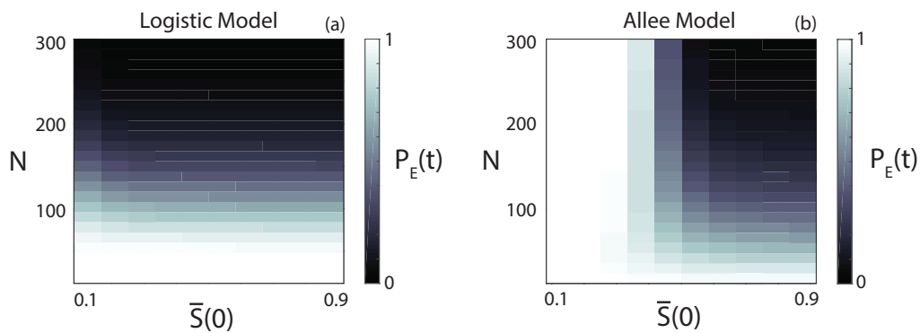
Figure 8. SSDA predictions for the probability of population extinction by (a) T_{\text{end}} = 2000 and (b) T_{\text{end}} = 10^4 for (a) the logistic model and (b) the Allee model. Parameters used are (a) P_m = 1 , P_b = 0.05 , P_d = 0.04 and (b) P_m = 1 , P_b^i = 0.02 , P_b^g = 0.015 , P_d^i = 0.04 , P_d^g = 0.005 .
