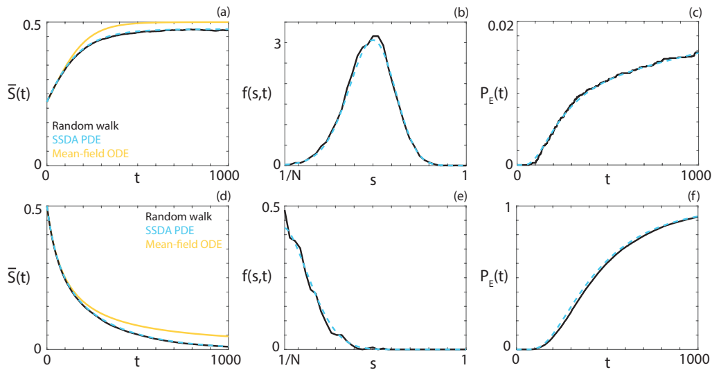
Figure 5. Comparison between the average behaviour of the lattice-based random walk (black), the SSDA PDE (cyan, dashed) and the mean-field ODE (orange) for the logistic growth model. (a),(d) The evolution of the average occupancy. (b),(e) The occupancy distribution probability density function. (c),(f) The evolution of the extinction probability. Parameters used are P_m = 1 , P_b = 0.02 , P_d = 0.01 , T_{\text{end}} = 1000 , N = 36 , N_0 = 8 and (d)-(f) P_m = 1 , P_b = 0.02 , P_d = 0.02 , T_{\text{end}} = 1000 , N = 36 , N_0 = 18 . Results are obtained from 10^4 identically-prepared realisations of the random walk.
