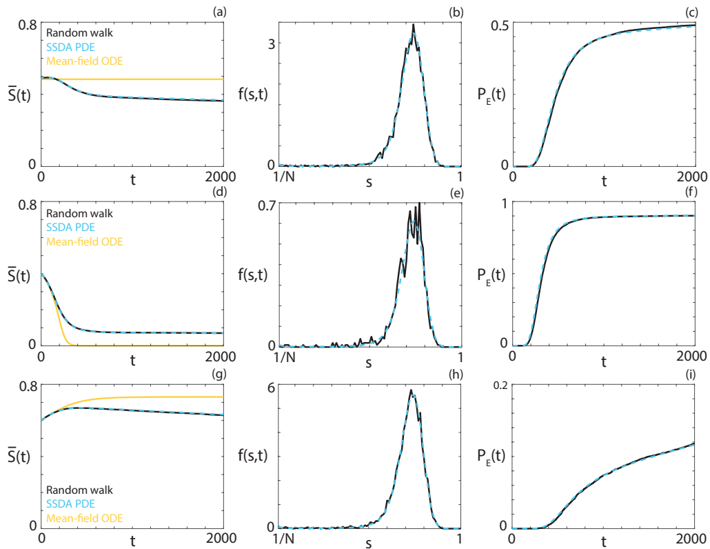
Figure 6. Comparison between the average behaviour of the lattice-based random walk (black), the SSDA PDE (cyan, dashed) and the mean-field ODE (orange) for the Allee model. (a),(d),(g) The evolution of the average occupancy. (b),(e),(h) The occupancy distribution probability density function. (c),(f),(i) The evolution of the extinction probability. Parameters used are P_m = 1 , P_b^i = 0.01 , P_b^g = 0.01 , P_d^i = 0.04 , P_d^g = 0.0025 , T_{\text{end}} = 2000 , N = 100 and (a)-(c) N_0 = 49 , (d)-(f) N_0 = 40 , (g)-(i) N_0 = 60 . Results are obtained from 10^4 identically-prepared realisations of the random walk.
