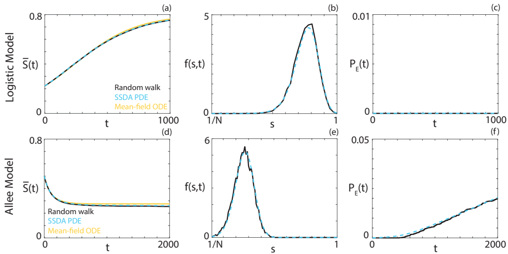
Figure 4. Comparison between the average behaviour of the lattice-based random walk (black), the SSDA PDE (cyan, dashed) and the mean-field ODE (orange) for the (a)-(c) logistic growth model and the (d)-(f) Allee model. (a),(d) The evolution of the average occupancy. (b),(e) The occupancy distribution probability density function. (c),(f) The evolution of the extinction probability. Parameters used are (a)-(c) P_m = 1 , P_b = 0.005 , P_d = 0.001 , T_{\text{end}} = 1000 , N = 36 , N_0 = 8 and (d)-(f) P_m = 1 , P_b^i = 0.03 , P_b^g = 0.01 , P_d^i = 0.02 , P_d^g = 0.01 , T_{\text{end}} = 2000 , N = 100 , N_0 = 50 . Results are obtained from 10^4 identically-prepared realisations of the random walk.
