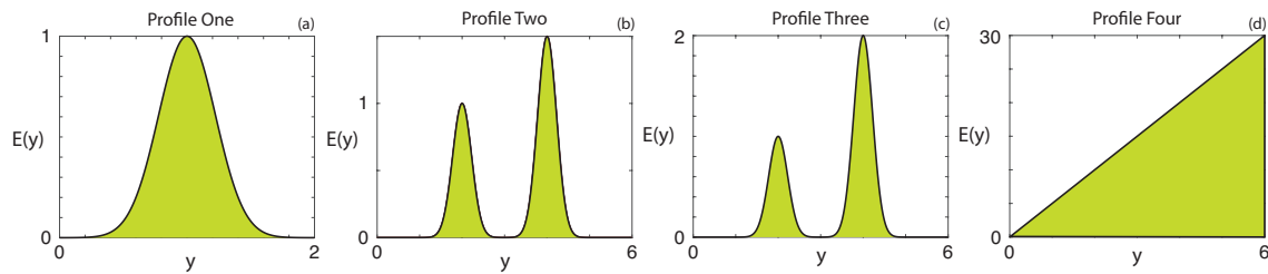
Figure 2: Four different idealised elevation profiles.
