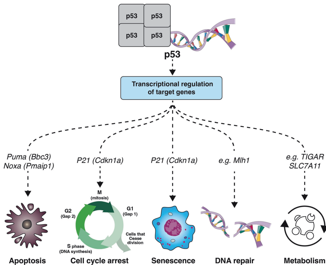
Fig. 1 Cellular processes regulated by p53. p53 regulates diverse cellular processes via the transcriptional regulation of target genes. Some cellular processes that contribute to the tumour suppressive function of p53 include apoptosis, cell cycle arrest, cell senescence, DNA repair and cell metabolism. Some genes essential for carrying out these processes are indicated.
