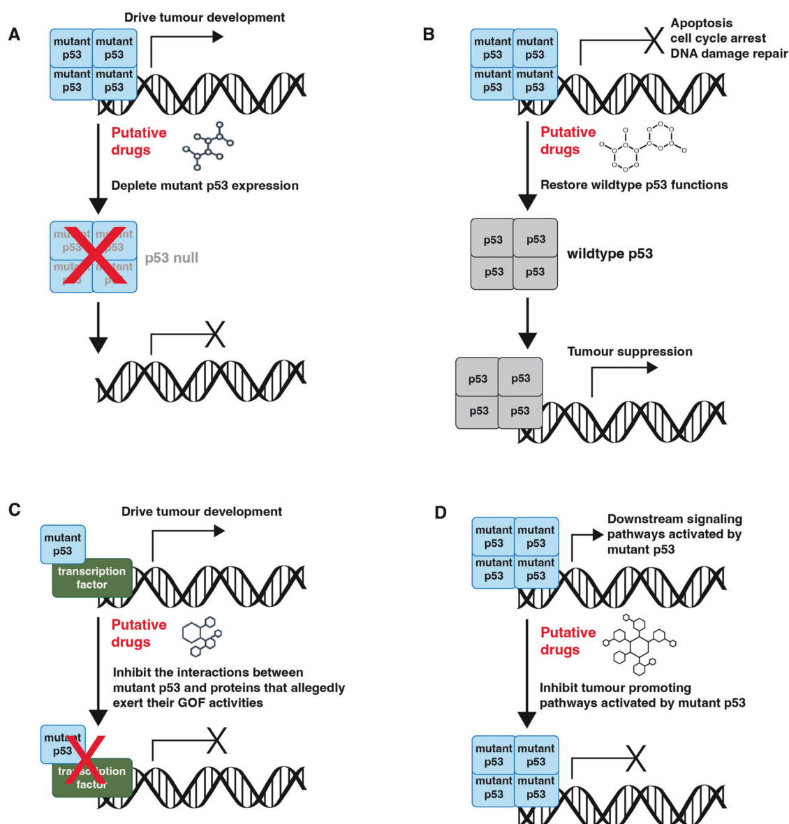
Fig. 4 Therapeutic strategies to target mutant p53 in cancer. A Promoting the degradation of mutant p53 proteins through proteasomal or autophagy pathways. B Restoring WT p53 function in mutant p53 proteins in cancer cells. C Inhibiting the interactions between mutant p53 and proteins that allegedly exert their GOF activities. D Inhibiting downstream signalling pathways that may be activated by mutant p53.
