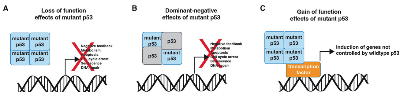
Fig. 2 Consequences of point mutation for p53 function. WT p53 proteins bind to DNA and activate the downstream signalling pathways. A Loss of function (LOF) effects of mutant p53 abrogate normal p53-mediated cellular processes. B Dominant negative effects (DNE) of mutant p53 are a consequence of mixed tetramers containing both WT and mutant p53 proteins, which are significantly less efficient at activating the WT p53 target genes compared to tetramers containing only WT p53. C Gain of function (GOF) effects of mutant p53 proteins are thought to be exerted by binding to and modulating the functions of transcription factors not bound and impacted by WT p53.
