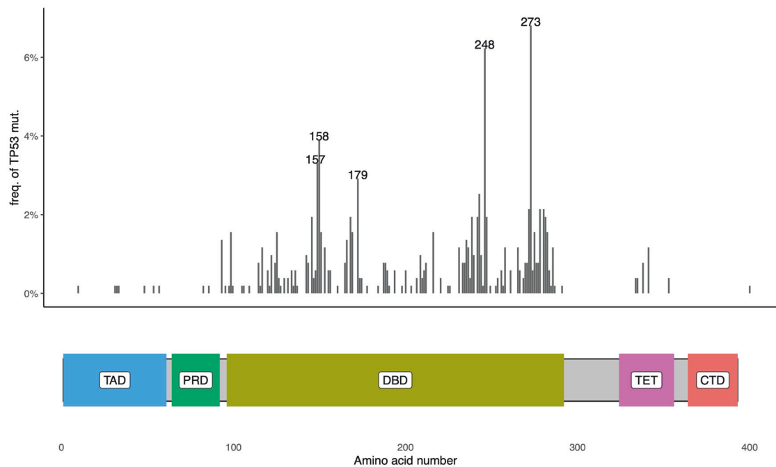
Fig. 3 p53 missense mutations in human LUAD. Frequencies of p53 mutants in LUAD patients with p53 missense mutations ( N = 514 ) were obtained from the GENIE BPC NSCLC v2.0 cohort [219], with domains of the p53 protein displayed below [220]. The protein schematic was generated using the drawProteins package [221]. TAD transactivation domain, PRD proline-rich domain, DBD DNA-binding domain, TET tetramerisation domain, CTD C-terminal regulatory domain.
