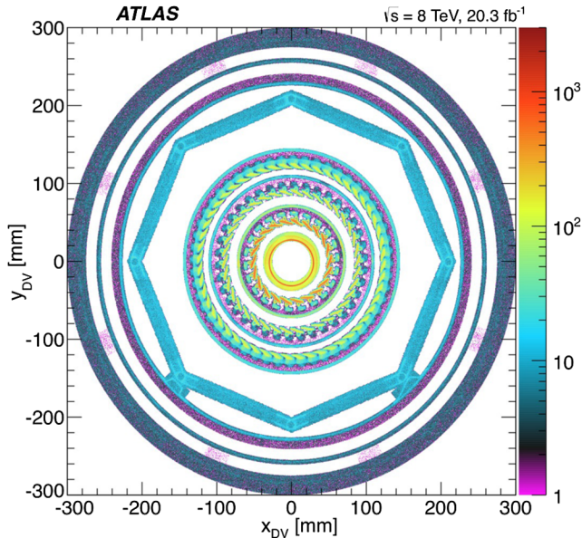
FIG. 2 (color online). Transverse-plane density (in arbitrary units) of vertices with fewer than five tracks in material regions that are excluded by the material veto in the region |z| < 300 mm. The innermost circle corresponds to the beam pipe. This is surrounded by the three pixel layers. The octagonal shape and outermost circles are due to support structures separating the pixel and SCT detectors.
