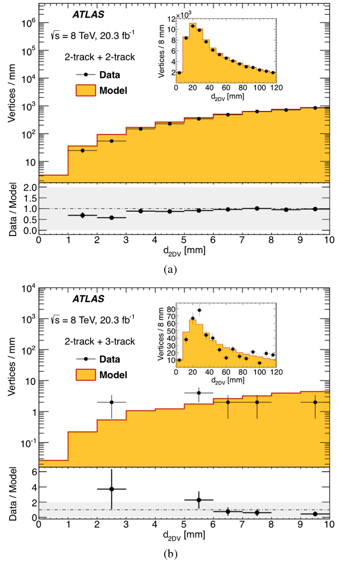
FIG. 7 (color online). The distribution of the distance d_{2DV} between (a) two 2-track vertices and (b) a 2-track vertex and a 3-track vertex with a combined mass above 10 GeV for the jets + E_T^{miss} stream data (data points) and in the model sample, in which the two vertices are in different events (histogram). A conservative 100% uncertainty on the model is shown in the data/model ratio plot. The inset shows the d_{2DV} distance up to values of 120 mm. The merged-vertex background estimate is determined from the area under the model distribution in the range d_{2DV} < 1 mm in (b).
