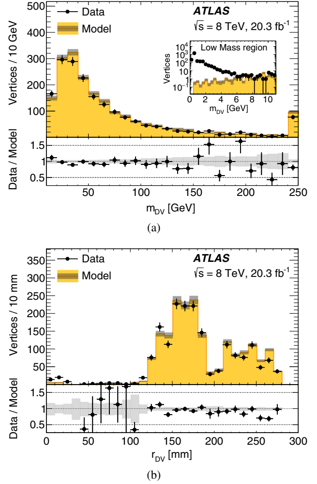
FIG. 8 (color online). Distributions of the (a) vertex mass and (b) vertex position radius for vertices composed of two nonlepton tracks in the data sample (data points), and the predicted model distribution obtained from vertices formed by combining tracks from two different data events (shaded histograms). The ratio of the data to the model distributions is shown below each plot. The gray bands indicate the statistical uncertainties for the predicted distributions. The inset shows the mass distribution in the low-mass region, elsewhere m_{DV} > 10 GeV is required. In (a), the highest bin shows the histogram overflow.
