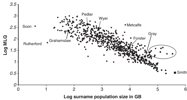
Figure 1 Graph of the log (MLQ) of the RD with the highest LQ for each surname ( y -axis) against log (surname population size) in the 1881 census ( x -axis). There are a number of surnames (circled) with a higher MLQ than might be expected for the surname sample size (Jones, Davies, Evans, Thomas, Hughes, James and Phillips), which are established Welsh surnames. The surnames from Supplementary Figure 1 are also marked.
