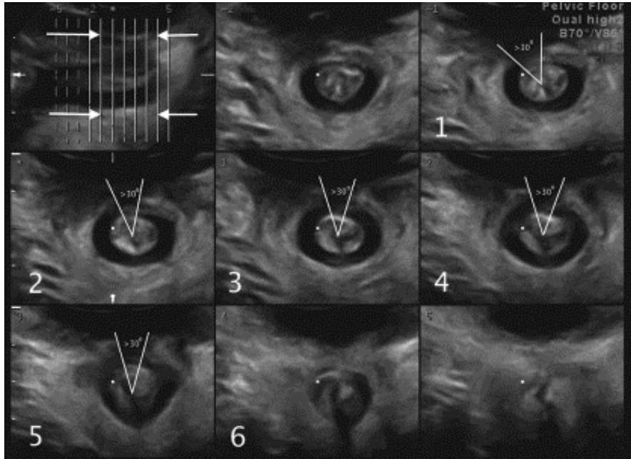
Figure 10: Assessment of the integrity of the anal sphincter complex assessed with tomographic ultrasound imaging plane (reproduced with permission from Guzman Rojas et al 165 ).
