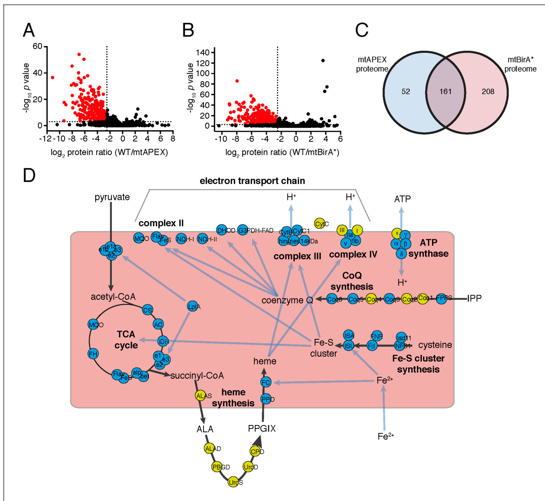
Figure 2. The mitochondrial proteome of T. gondii . (A–B) Volcano plots showing the log 2 protein ratios vs -\log_{10} p values of biotinylated proteins in WT compared to mtAPEX (WT/APEX) samples (A) and in WT compared to mtBirA* samples (WT/BirA*) (B) following the quantitative pipeline analysis. Proteins were deemed to be enriched in the mitochondrion if the log 2 fold change in protein expression was \leq -2.5 and the p value \leq 0.001 (red). (C) Venn diagram of the mtAPEX and mtBirA* proteomes. 161 proteins were identified in both proteomes, while 52 were unique to the mtAPEX proteome and 208 unique to the mtBirA* proteome. (D) Metabolic map of expected mitochondrial proteins (circles), showing proteins present (blue) and absent (yellow) from the T. gondii mitochondrial proteome. Black arrows represent the flow of metabolites through metabolic pathways in the mitochondrion, and blue arrows depict the flow of ions, minerals or metabolic pathway products.
