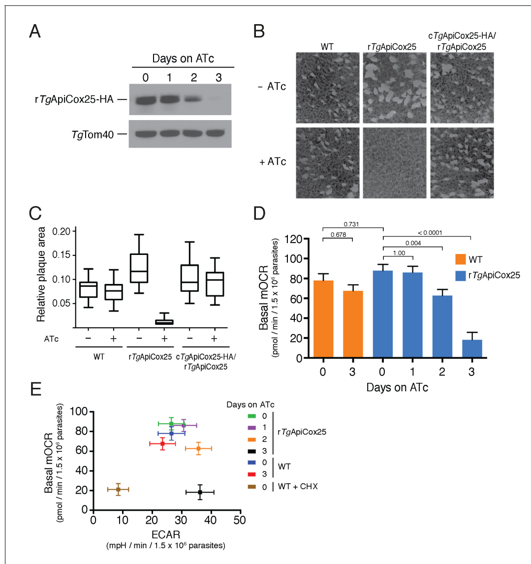
Figure 5. TgApiCox25 is important for parasite growth and mitochondrial O 2 consumption. (A) Western blot of proteins extracted from rTgApiCox25 -HA parasites grown in the absence of ATc, or in ATc for 1–3 days, and detected using anti-HA antibodies (top) and anti-TgTom40 (as a loading control; bottom). (B) Plaque assays measuring growth of WT, rTgApiCox25 and complemented cTgApiCox25 -HA/ rTgApiCox25 parasites cultured in the absence (top) or presence (bottom) of ATc. Assays are from a single experiment and are representative of 3 independent experiments. (C) Quantification of plaque size from WT, rTgApiCox25 and complemented cTgApiCox25 -HA/ rTgApiCox25 parasites grown in the absence or presence of ATc for 9 days. Box and whisker plots depict the median plaque size (centre line), the 25 th and 75 th percentiles (box) and the 5 th and 95 th percentiles (lines). Data are from 30 plaques per flask from a single experiment, except in the case of the rTgApiCox25 strain, where only 18 plaques were discernible. (D) Basal mitochondrial oxygen consumption rates (mOCR) in WT parasites grown in the absence of ATc or in the presence of ATc for 3 days (orange), and rTgApiCox25 parasites grown in the absence of ATc, or in the presence of ATc for 1–3 days (blue). A linear mixed-effects model was fitted to the data, and the values depict the mean \pm s.e.m. from three independent experiments. A one-way ANOVA followed by Tukey's multiple pairwise comparison test was performed. Relevant p values are shown. (E) Basal mOCR plotted against basal extracellular acidification rate (ECAR) of WT cells grown in the absence of ATc, the presence of cycloheximide (CHX) for 1 day, or the presence of ATc for 3 days, and rTgApiCox25 parasites grown in the absence of ATc or presence of ATc for 1–3 days (mean \pm s.e.m. of the linear mixed-effects model described above; n = 3).
