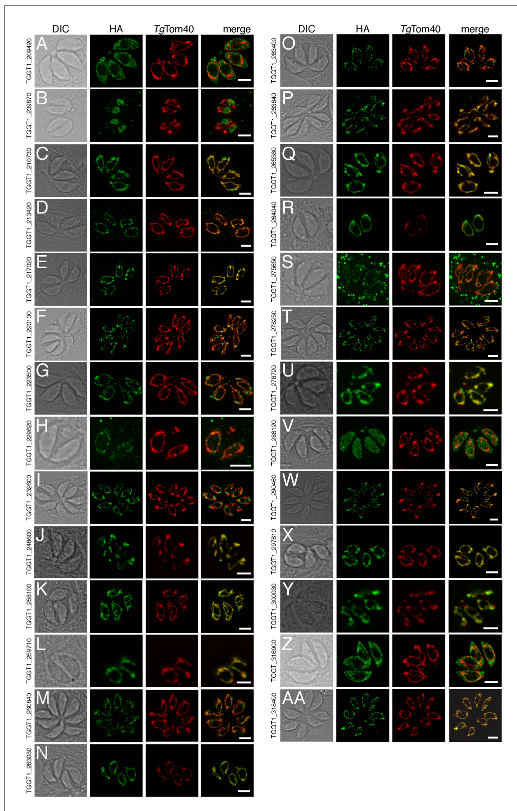
Figure 3. The localization of novel proteins from the T. gondii mitochondrial proteome. (A–AA) Proteins with no previously determined localization in T. gondii were selected from the mitochondrial proteome, and the corresponding gene was tagged at the 3'-terminus of the open reading frame with a HA tag. Immunofluorescence assays depict HA-tagged proteins (green) co-labelled with the mitochondrial marker TgTom40 (red). The http://toxodb.org gene identification number is depicted for every gene that was tagged.
