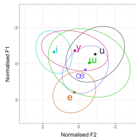
Figure 4. Normalised mean F1 and F2 values for L2 Turkish vowels for all speakers combined. Each ellipse includes approximately 95% of the samples in each vowel category.
