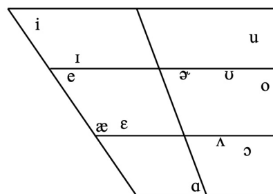
Figure 1. American English vowels in Northern Cities dialect regions according to Hillenbrand (2003) .
