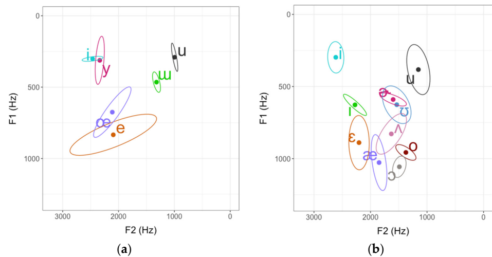
Figure 7. (a) Mean F1 and F2 values for L2 Turkish vowels produced by speaker F39. Each ellipse includes approximately 95% of the samples in each vowel category. (b) Mean F1 and F2 values for L1 English vowels produced by speaker F39. Each ellipse includes approximately 95% of the samples in each vowel category.
