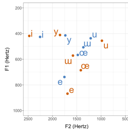
Figure 3. Mean F1 and F2 values for the vowels /i y e œ u/ produced by L1 AmE speakers (in blue), superimposed over the mean F1 and F2 values for the vowels produced by a native female speaker of Standard Istanbul Turkish (in orange).
