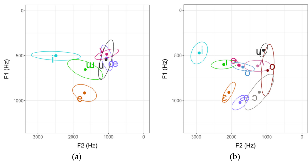
Figure 8. (a) Mean F1 and F2 values for L2 Turkish vowels produced by speaker F07. Each ellipse includes approximately 95% of the samples in each vowel category. (b) Mean F1 and F2 values for L1 English vowels produced by speaker F07. Each ellipse includes approximately 95% of the samples in each vowel category.
