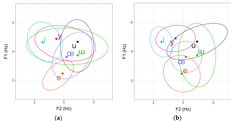
Figure 5. (a) Mean F1 and F2 values for L2 Turkish vowels produced by the speakers in the urban group. Each ellipse includes approximately 95% of the samples in each vowel category. (b) Mean F1 and F2 values for L2 Turkish vowels produced by the speakers in the regional group. Each ellipse includes approximately 95% of the samples in each vowel category.
