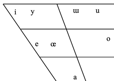
Figure 2. Standard Istanbul Turkish vowels according to Zimmer and Orgun (1992).
