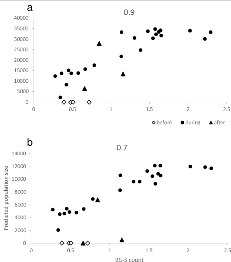
Fig. 3 Observed density of females in the Tri Nguyen population during the release from BG-S counts (x axis) plotted against predicted numbers of release individuals present in the population (y axis) based on two values of daily mortality, (a) 0.9 and (b) 0.7. BG-S counts before the first release and predicted numbers after releases finished (but when released individuals were still expected to be present in the population) are also presented
