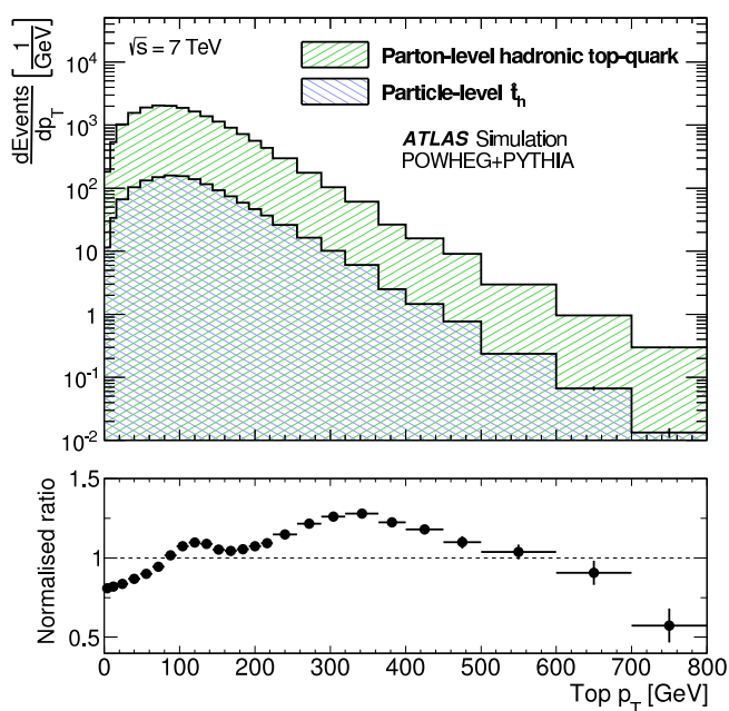
Figure 1. Simulated event distribution of the parton-level top-quark p_T distribution for all events (green), and the particle-level pseudo-top-quark p_T ( \hat{t}_h ) for events within the fiducial region (blue). In both cases the top-quark that decays hadronically is chosen. The distributions are evaluated for the same event sample based on POWHEG+PYTHIA at \sqrt{s} = 7 TeV. The upper figure is made for an arbitrary integrated luminosity. The lower figure shows the ratio of the particle-level \hat{t}_h over the parton-level top-quark normalised distributions to emphasise the difference in shape between the two.
