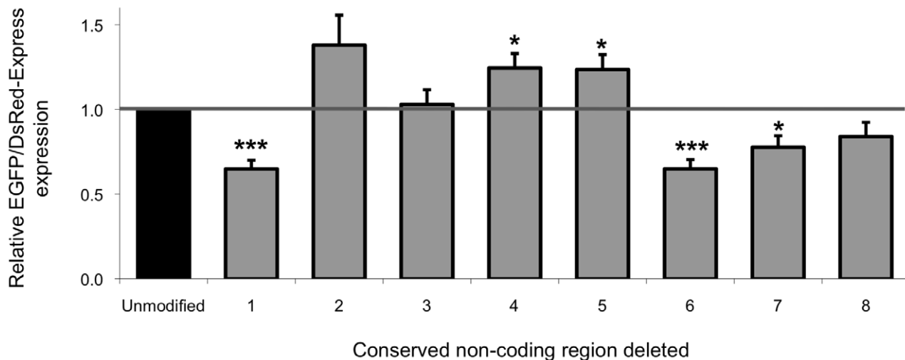
Figure 2. Expression analysis of BAC dual-reporter deletion constructs. BHK-21 cells were transfected with the RP11-265B8::Ex5a-EK-DsAmp (Dual Reporter) construct and derivatives individually containing deletions of the identified conserved non-coding regions. EGFP and DsRed-Express expression were measured by flow cytometry 72 hours post transfection. The expression of the different deletion constructs was compared to the expression of the control RP11-265B8::Ex5a-EK-DsAmp (Dual Reporter) construct. Assays were performed in triplicate on at least three independent occasions. Error bars represent standard error of the mean. * p < 0.05 , *** p < 0.001 in comparison to the unmodified control RP11-265B8::Ex5a-EK-DsAmp (Dual Reporter) construct. doi:10.1371/journal.pone.0022001.g002
