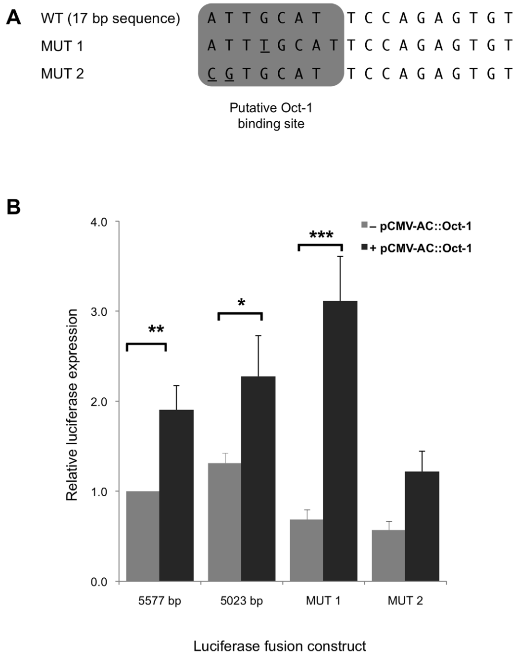
Figure 7. Regulatory effects of a putative Oct-1 binding site located within conserved region 1. (A) Two mutant constructs were generated by site directed mutagenesis within a putative Oct-1 binding site within the identified 17 bp nucleotide sequence. MUT 1 contains one additional extra base in the middle of the sequence and MUT 2 contains two bases substitution at the start of the sequence. (B) MUT 1 and MUT 2 were generated in the pGL3-Basic::5023 construct. Luciferase expression of the mutant constructs was analyzed following co-transfection of BE(2)-M17 cells with pGL3-Basic derivatives and Oct-1 transcription factor-encoding plasmid pCMV-AC::Oct-1. The overall levels of expression were then compared to the pGL3-Basic::5577 vector, the expression value of which was set as 1. Assays were performed in triplicate on at least three independent occasions. Error bars represent standard error of the mean. * p < 0.05 ; ** p < 0.01 ; *** p < 0.001 . doi:10.1371/journal.pone.0022001.g007
