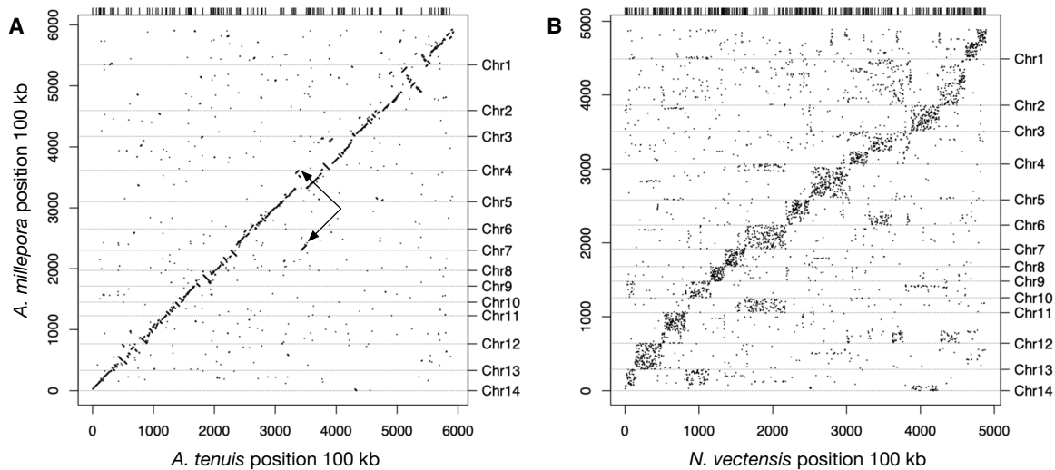
Fig. 1. Macrosyntenic conservation between A. tenuis and other cnidarian genomes. Dots represent blocks of collinear groups of genes and margin lines represent boundaries between contigs (top) or A. millepora linkage groups (right). In (A), very few A. tenuis scaffolds map across A. millepora chromosomes (a single example is shown with arrows). In (B), the blocks along the diagonal reflect ancient conserved linkage groups that roughly correspond to chromosomes in A. millepora .
