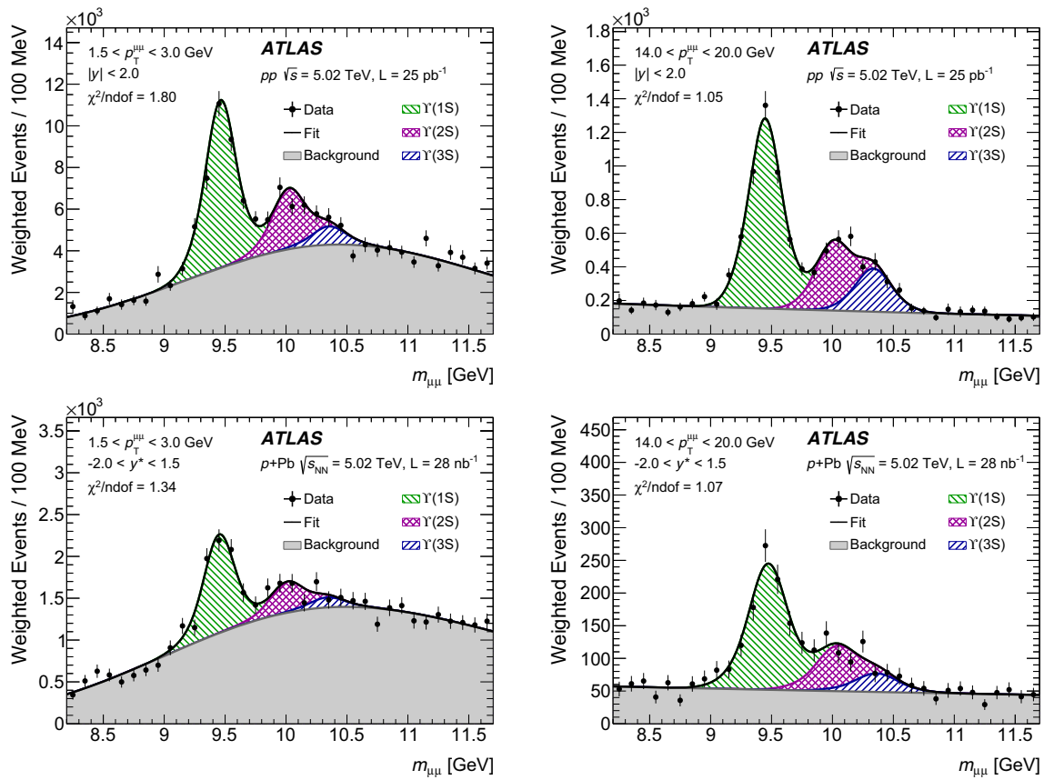
Fig. 2 Bottomonium fit results in dimuon invariant mass m_{\mu\mu} for pp collisions at \sqrt{s} = 5.02 TeV (top) and p+\text{Pb} collisions at \sqrt{s_{\text{NN}}} = 5.02 TeV (bottom) for one typical low p_{\text{T}}^{\mu\mu} interval of 1.5 < p_{\text{T}}^{\mu\mu} < 3.0 GeV (left) and one high p_{\text{T}}^{\mu\mu} interval of 14 < p_{\text{T}}^{\mu\mu} < 20 GeV (right). For all the shown fits, \Upsilon(1\text{S}) acceptance weights are assigned. The goodness of the bottomonium fit with \text{ndof} = 24 is also presented
