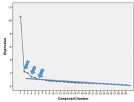
Figure 1. Scree Plot of eigenvalues of components for Principal Component Analysis. Three arrows and a line were added to show the points of inflexion at component 2, 4 and 6.
