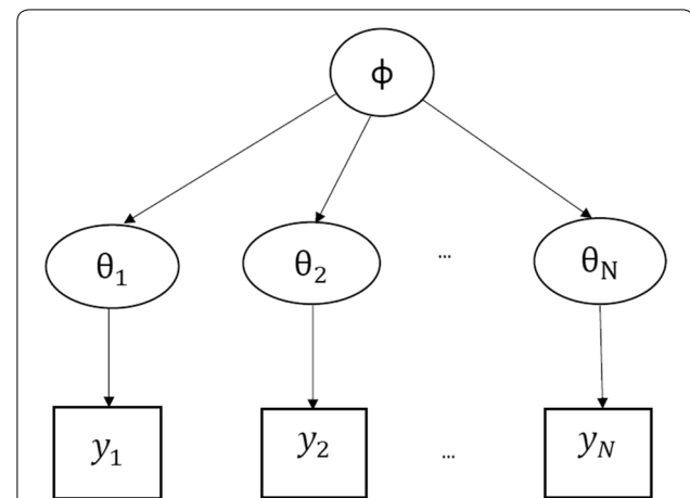
Fig. 1 An example hierarchical model where the parameter \theta_i describes the probability distribution of the outcome y_i for subject i . In this graphical model, an arrow from a to b indicates that b is generated via a through a distribution p_a(b) , or in other words, a describes the distribution of b . The main part of this hierarchical model is that \theta_i 's are themselves assumed to be draws from a common distribution described by a hyperparameter \phi , which within a Bayesian framework, has its own prior distribution
