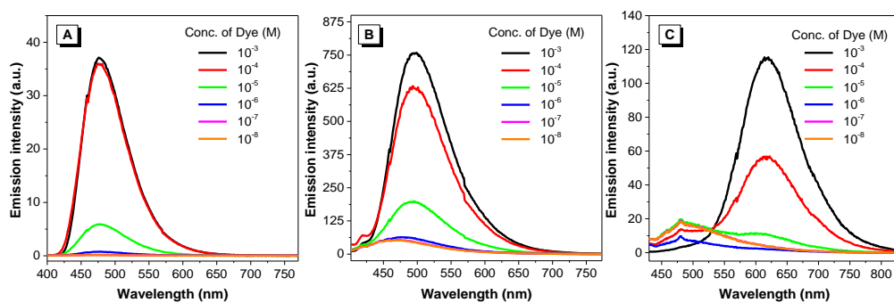
Figure 7. Emission spectra of dyes 1 (A), 2 (B) and 3 (C) at various concentrations in DMSO. Excitation wavelength: 390, 392 and 420 nm, respectively.
