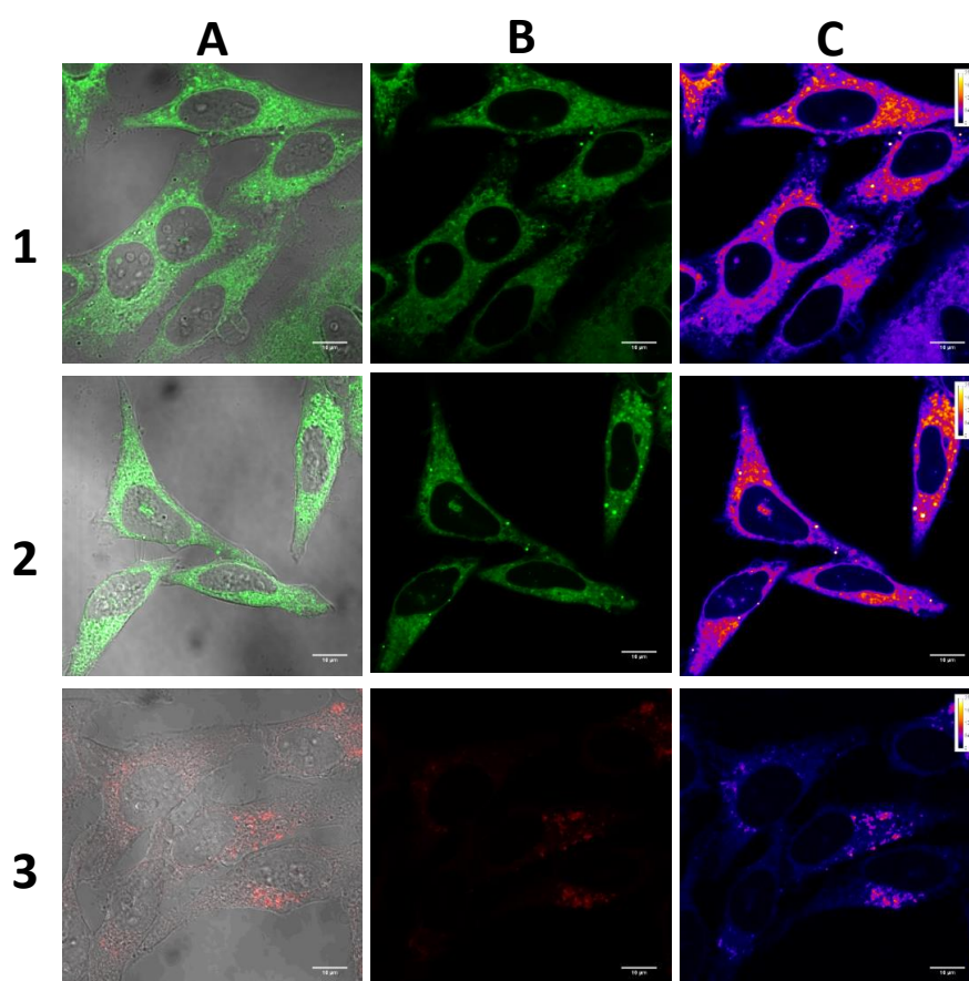
Figure 13. Confocal fluorescence microscopy image of HeLa cells stained with dyes 1 , 2 and 3 (10 \mu M) for 30 min. (A) Merged image of the fluorescence and bright-field images; (B) fluorescence image under excitation of 405 nm laser (2.0% for dyes 1 and 2 , 6.0% for dye 3 ); (C) the intensity of the signal was visualised using the “Fire” lookup table (LUT) colour scheme in Image J2. Linear mapping of pixel values in the display range indicated by the calibration bar (0–255 a.u.). Scale bar: 15 \mu m.
