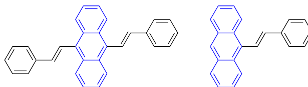
Figure 1. The structures of distyrylanthracene (left) and mono-functionalize anthracene (right).
