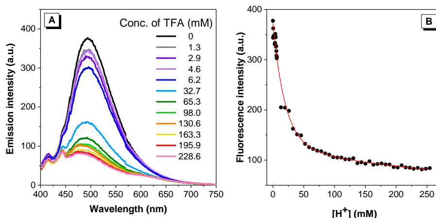
Figure 11. (A) Emission spectra of dye 2 in DMSO with increasing concentration of TFA. Dye concentration = 20 \mu\text{M} ; \lambda_{\text{ex}} : 392 nm; (B) emission intensity of dye 2 vs. proton concentration.
