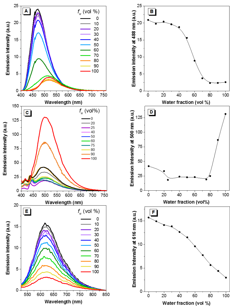
Figure 8. Emission intensity of dyes 1 (A,B), 2 (C,D) and 3 (E,F) in methanol/water mixtures with different water fractions. Concentration = 10 \mu M. f_w and vol% = water fraction. \lambda_{ex} : 385, 387 and 437 nm respectively.
