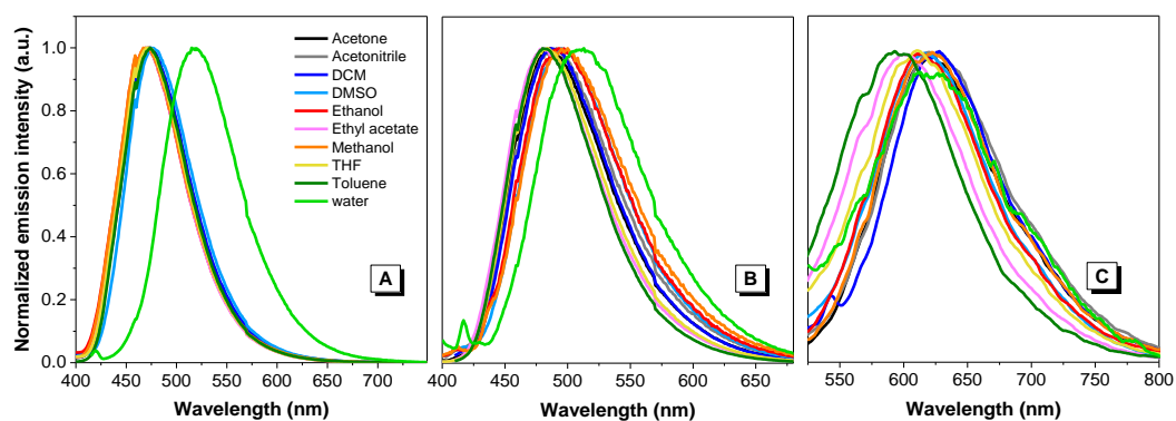
Figure 4. Normalized emission spectra of dyes 1 (A), 2 (B) and 3 (C) in different solvents. Concentration = 10 \mu M.
