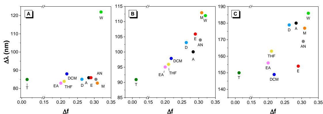
Figure 5. Lippert–Mataga solvatochromism plot of dyes 1 (A), 2 (B) and 3 (C) in different solvents as a function of solvent polarity measured by Lippert–Mataga polarity parameter. A = acetone, AN = acetonitrile, D = DMSO, E = ethanol, EA = ethyl acetate, M = methanol, T = toluene, W = water.
