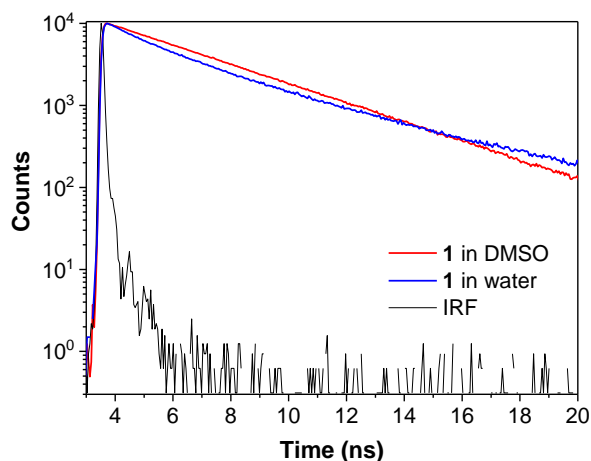
Figure 10. Fluorescence decay profile of dye 1 in DMSO (red) and water (blue). The black line shows the instrument response function (IRF) of the measurement system. Dye concentration: 10 \mu M. \lambda_{\text{ex}} : 400 nm. \lambda_{\text{em}} : 480 nm for DMSO and 520 nm for water.
