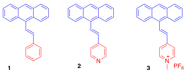
Figure 2. Chemical structures of dyes 1–3.
