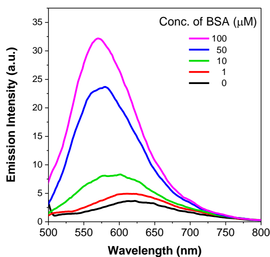
Figure 12. Fluorescence emission spectra of dye 3 with various concentrations of BSA in phosphate-buffered saline (PBS) excited at 420 nm.
