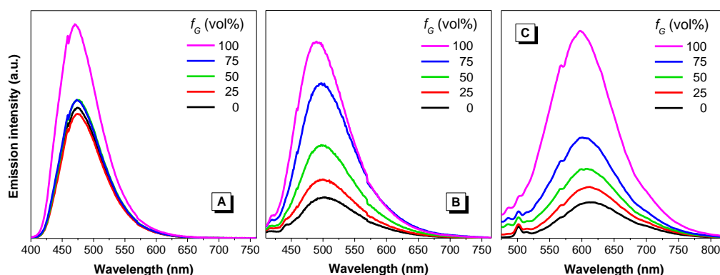
Figure 6. Emission spectra of dyes 1 (A), 2 (B) and 3 (C) in ethylene glycol/glycerol mixtures, where f_G indicates glycerol fraction. Concentration = 10 \mu M. Excitation wavelength: 388, 390 and 437 nm, respectively. Note: in panel C, the peak at approx. 500 nm corresponds to the Raman scattering of the solvent.
