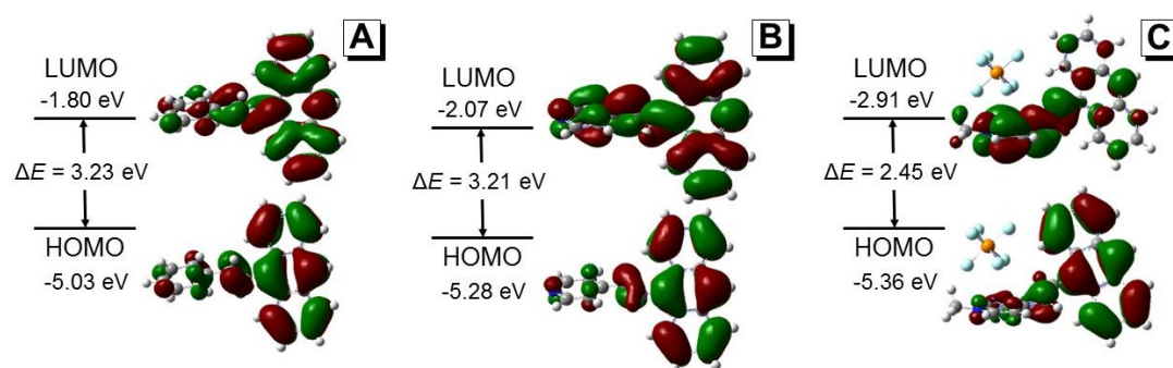
Figure 9. Molecular orbital amplitude plots and the HOMO/LUMO energy levels of 1 (A); 2 (B) and 3 (C) calculated using the B3LYP/6-31G basis set.
