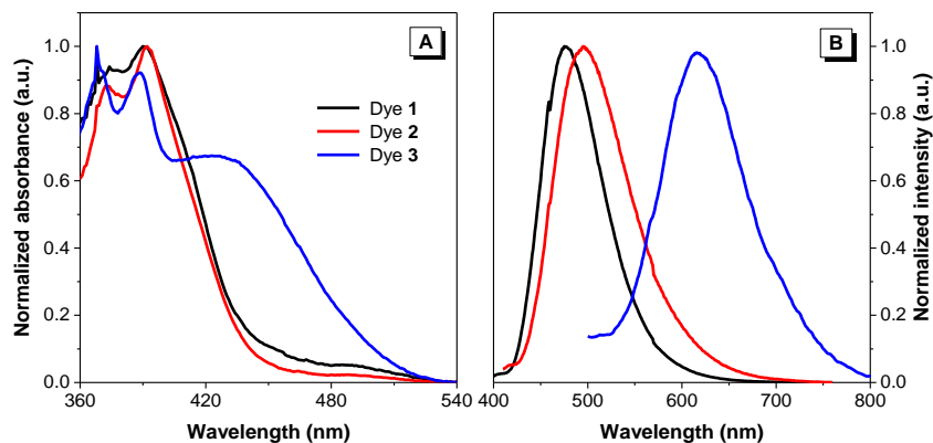
Figure 3. (A) Normalized absorption and (B) emission spectra in DMSO. Concentration = 10 \mu\text{M} . Excitation wavelength: 390 (1), 392 (2) and 420 nm (3).
